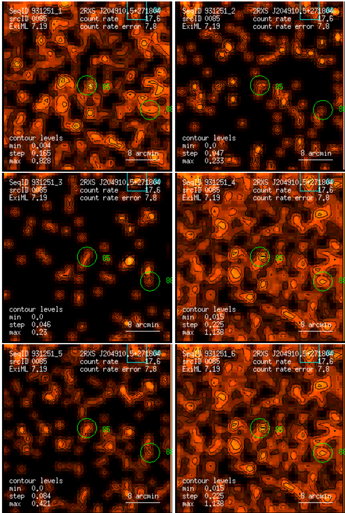
Figure 85: RASS 931251: detection 0085: band rate images, Gaussian filter: (1) PSPC channels 11 – 41, (2) 52 – 90, (3) 91 – 201, (4) 11 – 235, (5) 52 – 201, (6) 11 – 201. Broad band rates in counts/ks. Band rate contour levels in counts/ks/arcmin 2 .
