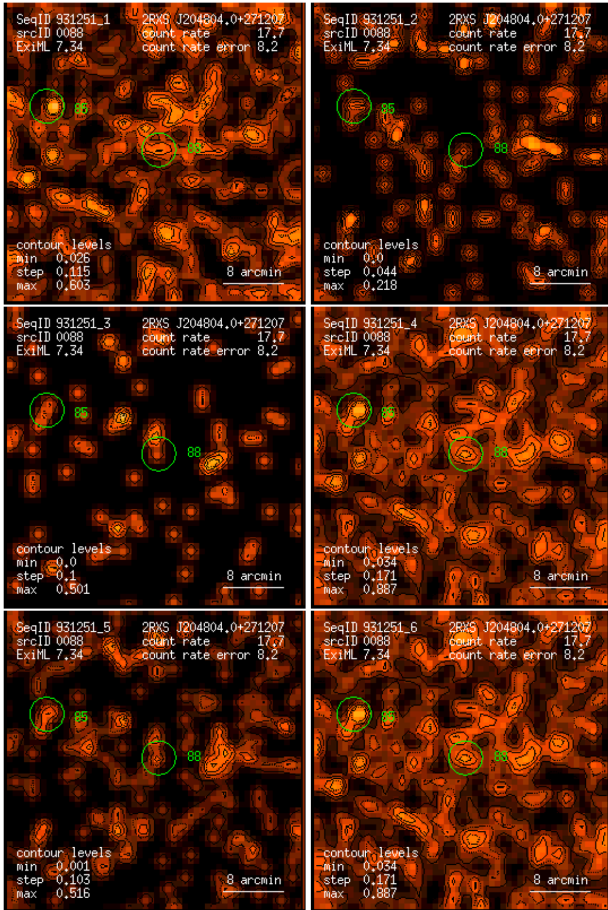
Figure 88: RASS 931251: detection 0088: band rate images, Gaussian filter: (1) PSPC channels 11 – 41, (2) 52 – 90, (3) 91 – 201, (4) 11 – 235, (5) 52 – 201, (6) 11 – 201. Broad band rates in counts/ks. Band rate contour levels in counts/ks/arcmin 2 .
