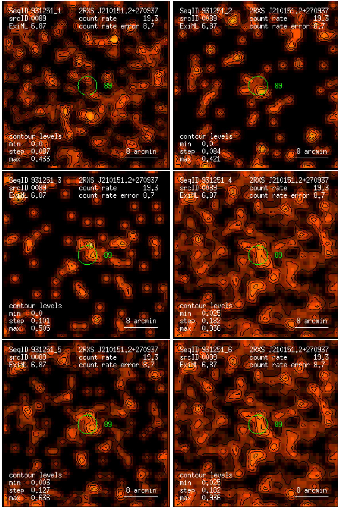
Figure 89: RASS 931251: detection 0089: band rate images, Gaussian filter: (1) PSPC channels 11 – 41, (2) 52 – 90, (3) 91 – 201, (4) 11 – 235, (5) 52 – 201, (6) 11 – 201. Broad band rates in counts/ks. Band rate contour levels in counts/ks/arcmin 2 .
