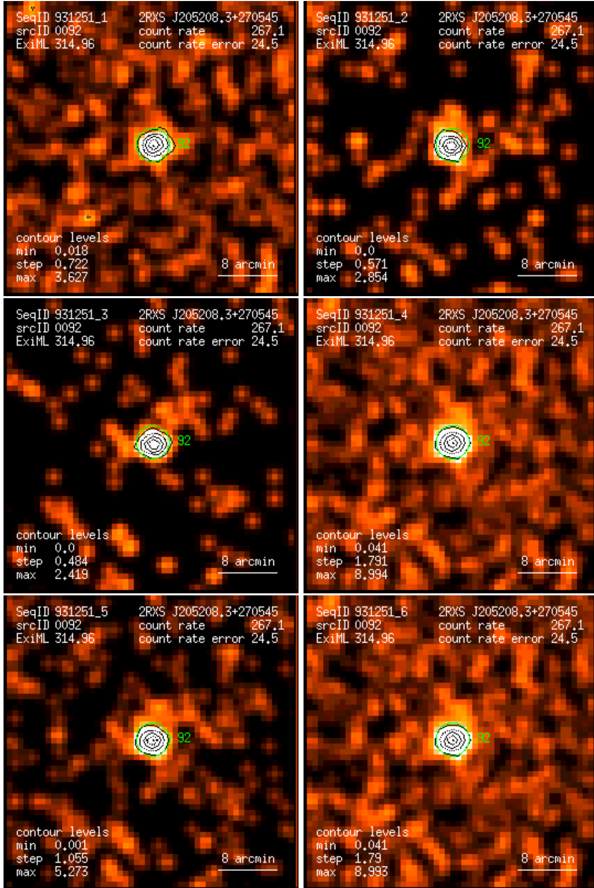
Figure 92: RASS 931251: detection 0092: band rate images, Gaussian filter: (1) PSPC channels 11 – 41, (2) 52 – 90, (3) 91 – 201, (4) 11 – 235, (5) 52 – 201, (6) 11 – 201. Broad band rates in counts/ks. Band rate contour levels in counts/ks/arcmin 2 .
