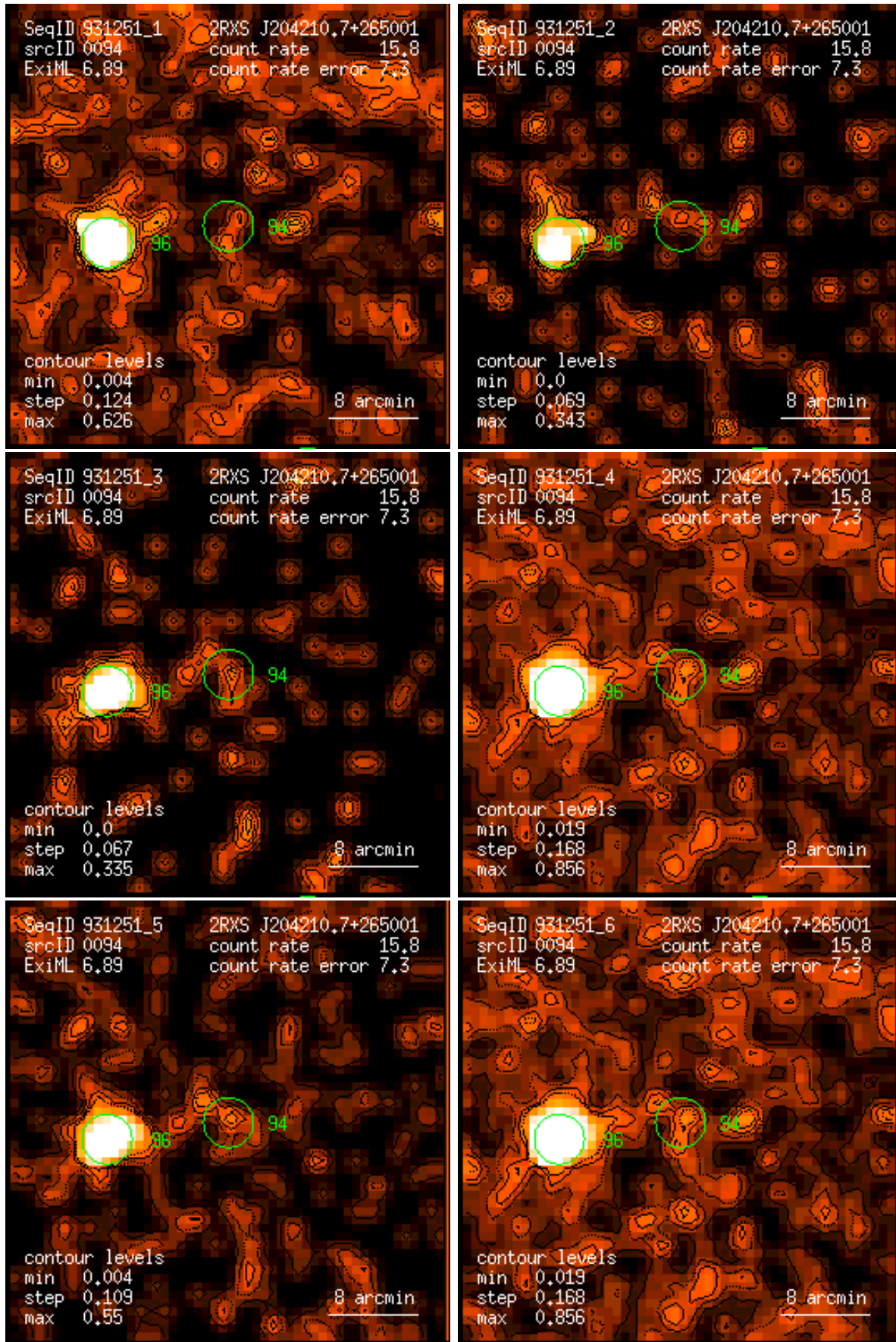
Figure 94: RASS 931251: detection 0094: band rate images, Gaussian filter: (1) PSPC channels 11 – 41, (2) 52 – 90, (3) 91 – 201, (4) 11 – 235, (5) 52 – 201, (6) 11 – 201. Broad band rates in counts/ks. Band rate contour levels in counts/ks/arcmin 2 .
