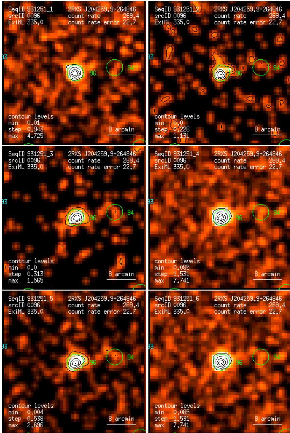
Figure 96: RASS 931251: detection 0096: band rate images, Gaussian filter: (1) PSPC channels 11 – 41, (2) 52 – 90, (3) 91 – 201, (4) 11 – 235, (5) 52 – 201, (6) 11 – 201. Broad band rates in counts/ks. Band rate contour levels in counts/ks/arcmin 2 .
