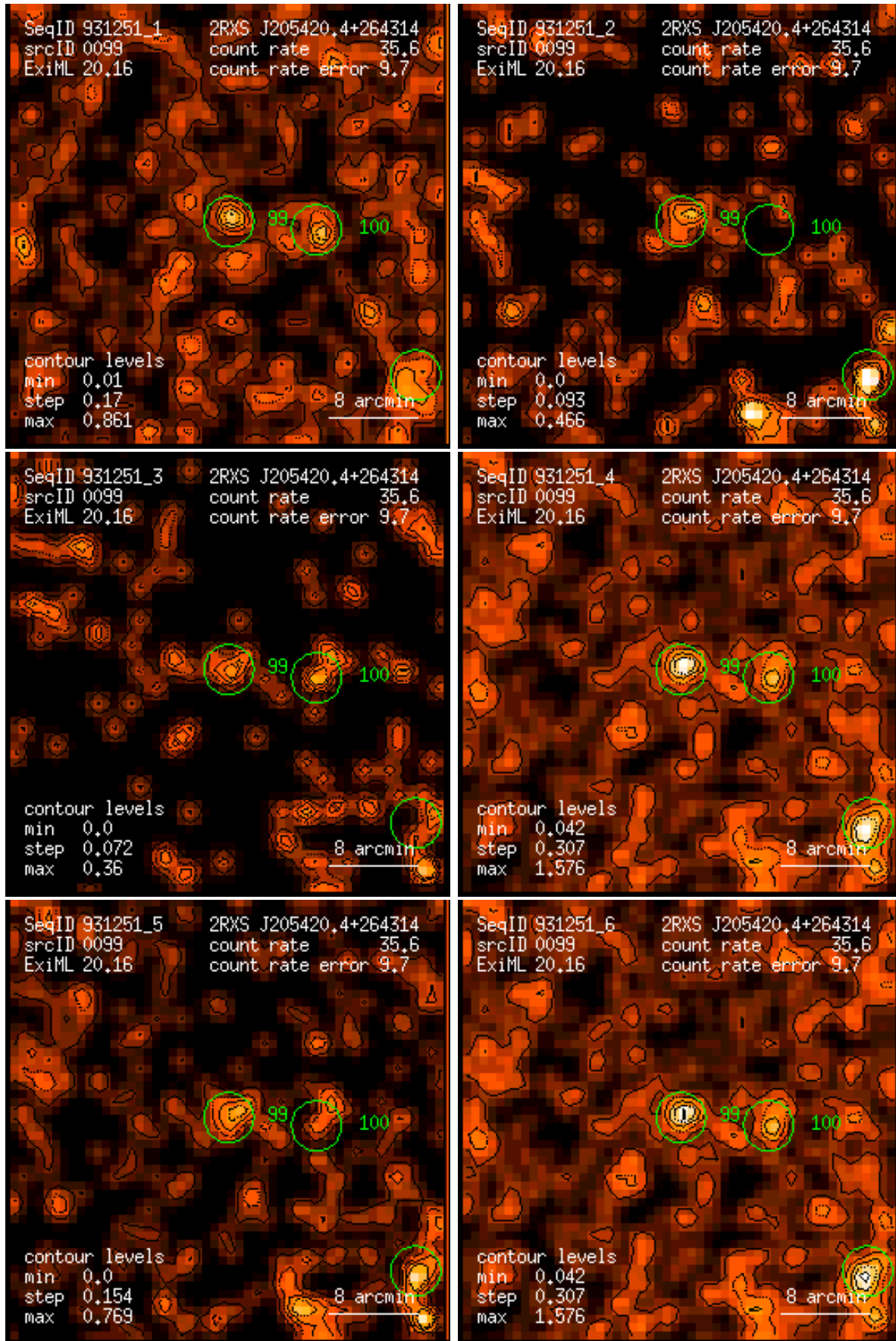
Figure 99: RASS 931251: detection 0099: band rate images, Gaussian filter: (1) PSPC channels 11 – 41, (2) 52 – 90, (3) 91 – 201, (4) 11 – 235, (5) 52 – 201, (6) 11 – 201. Broad band rates in counts/ks. Band rate contour levels in counts/ks/arcmin 2 .
