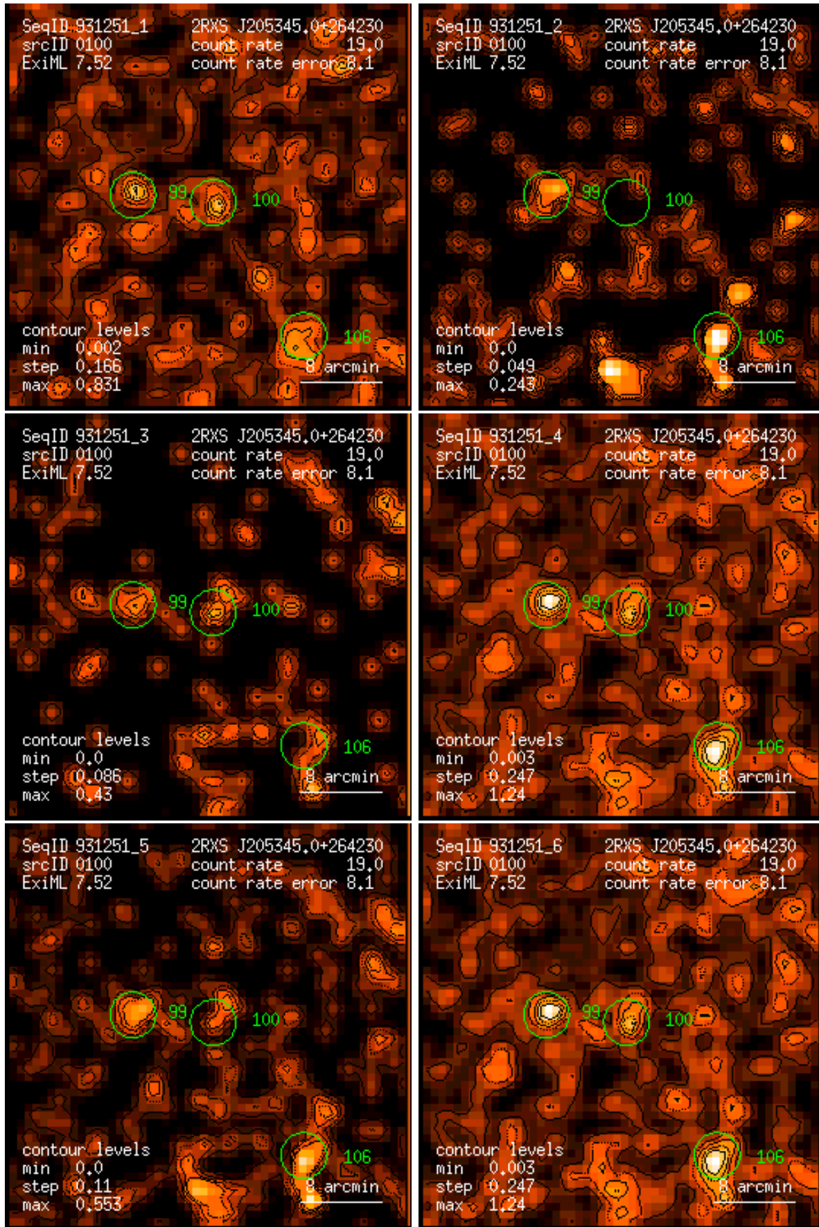
Figure 100: RASS 931251: detection 0100: band rate images, Gaussian filter: (1) PSPC channels 11 – 41, (2) 52 – 90, (3) 91 – 201, (4) 11 – 235, (5) 52 – 201, (6) 11 – 201. Broad band rates in counts/ks. Band rate contour levels in counts/ks/arcmin 2 .
