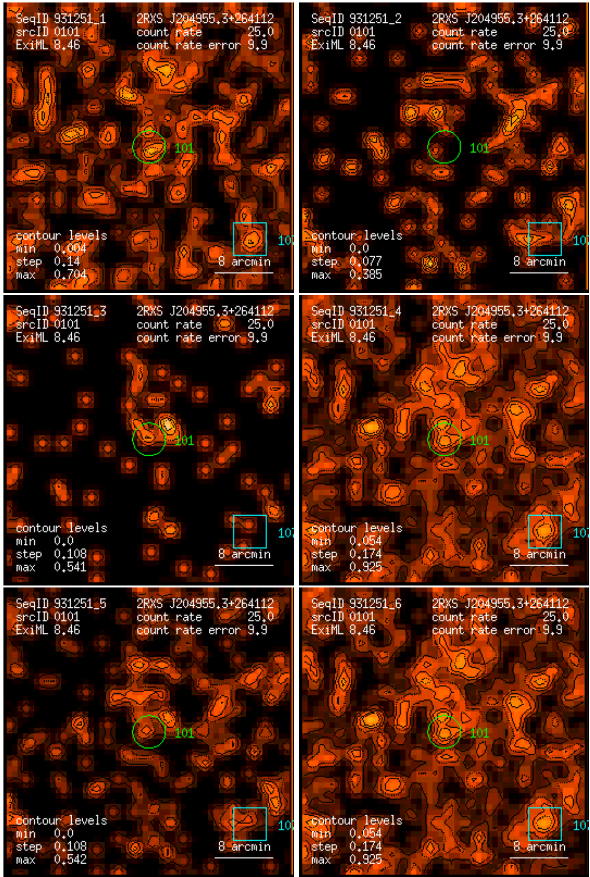
Figure 101: RASS 931251: detection 0101: band rate images, Gaussian filter: (1) PSPC channels 11 – 41, (2) 52 – 90, (3) 91 – 201, (4) 11 – 235, (5) 52 – 201, (6) 11 – 201. Broad band rates in counts/ks. Band rate contour levels in counts/ks/arcmin 2 .
