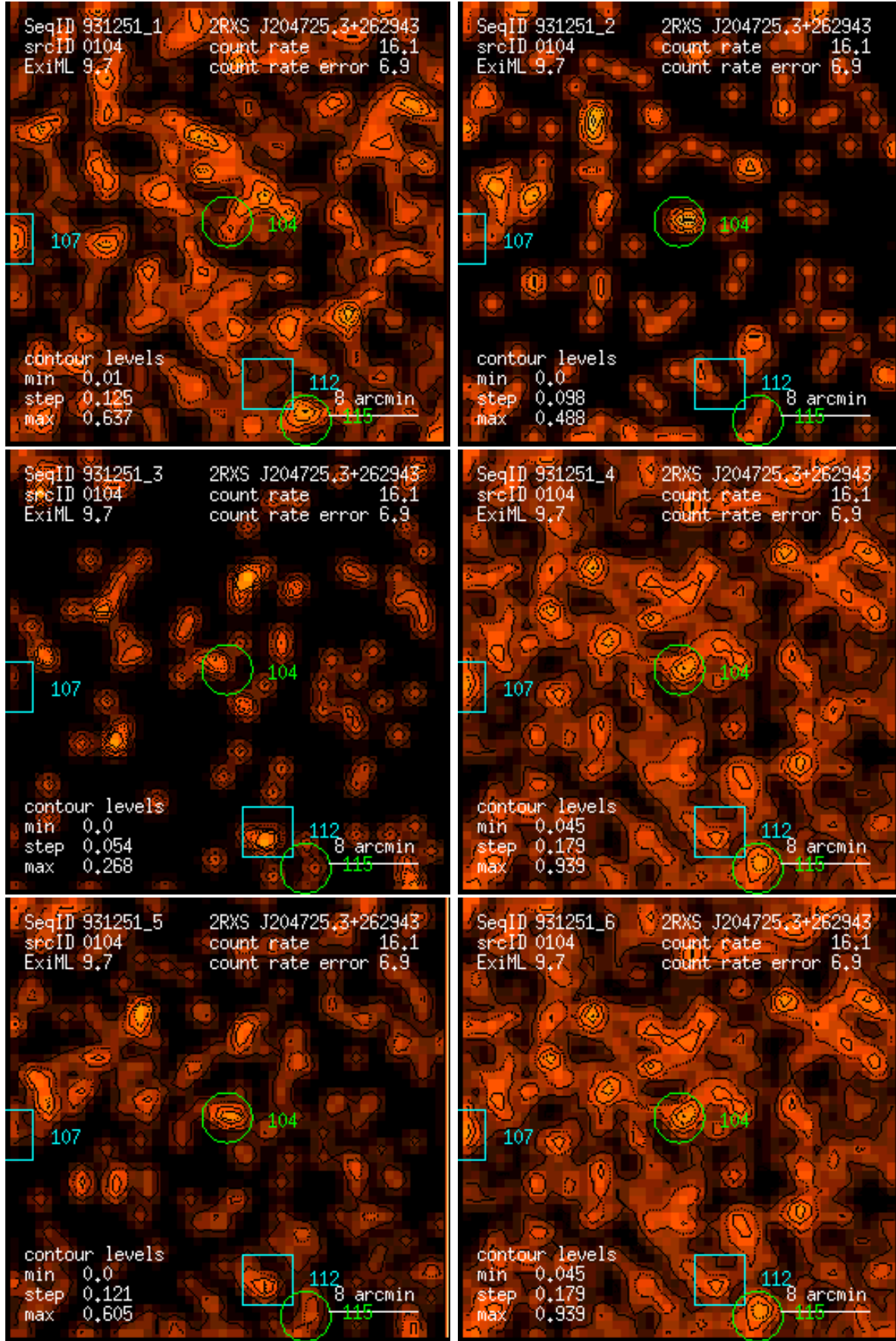
Figure 104: RASS 931251: detection 0104: band rate images, Gaussian filter: (1) PSPPC channels 11 – 41, (2) 52 – 90, (3) 91 – 201, (4) 11 – 235, (5) 52 – 201, (6) 11 – 201. Broad band rates in counts/ks. Band rate contour levels in counts/ks/arcmin 2 .
