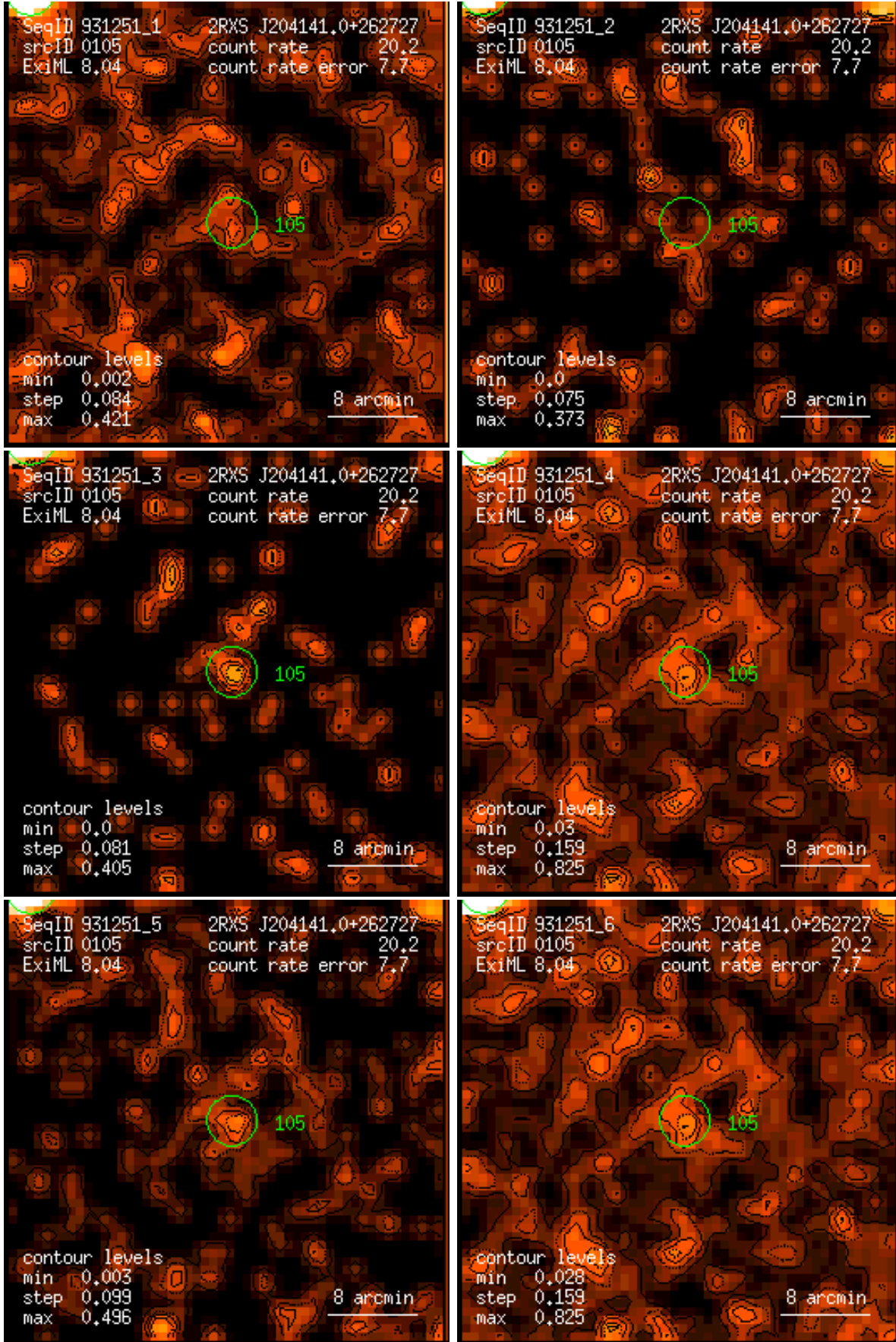
Figure 105: RASS 931251: detection 0105: band rate images, Gaussian filter: (1) PSPC channels 11 – 41, (2) 52 – 90, (3) 91 – 201, (4) 11 – 235, (5) 52 – 201, (6) 11 – 201. Broad band rates in counts/ks. Band rate contour levels in counts/ks/arcmin 2 .
