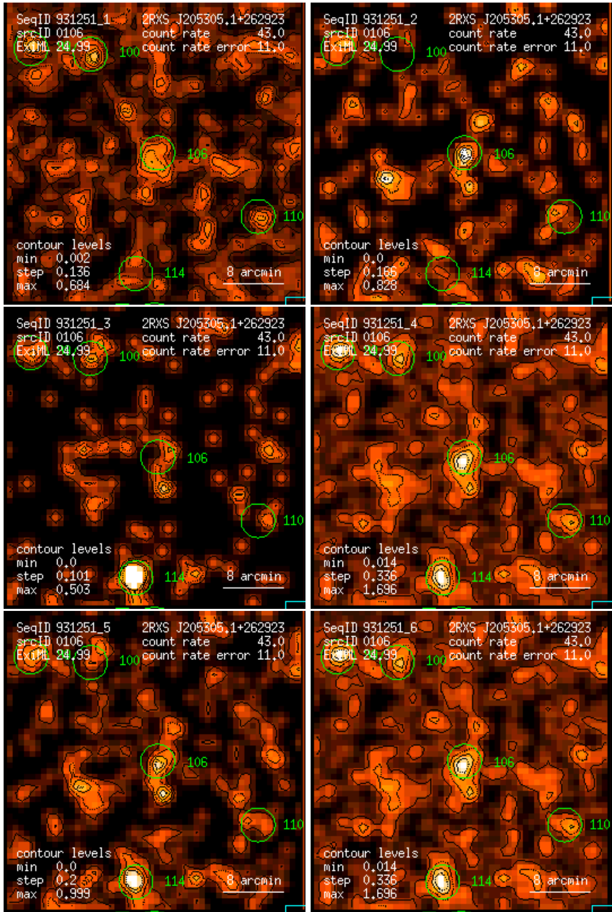
Figure 106: RASS 931251: detection 0106: band rate images, Gaussian filter: (1) PSPC channels 11 – 41, (2) 52 – 90, (3) 91 – 201, (4) 11 – 235, (5) 52 – 201, (6) 11 – 201. Broad band rates in counts/ks. Band rate contour levels in counts/ks/arcmin 2 .
