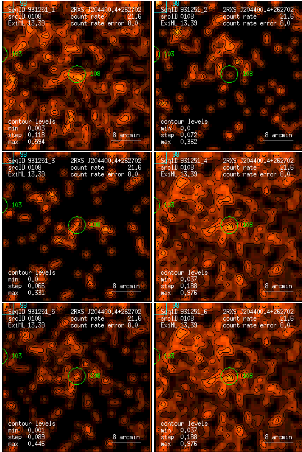
Figure 108: RASS 931251: detection 0108: band rate images, Gaussian filter: (1) PSPC channels 11 – 41, (2) 52 – 90, (3) 91 – 201, (4) 11 – 235, (5) 52 – 201, (6) 11 – 201. Broad band rates in counts/ks. Band rate contour levels in counts/ks/arcmin 2 .
