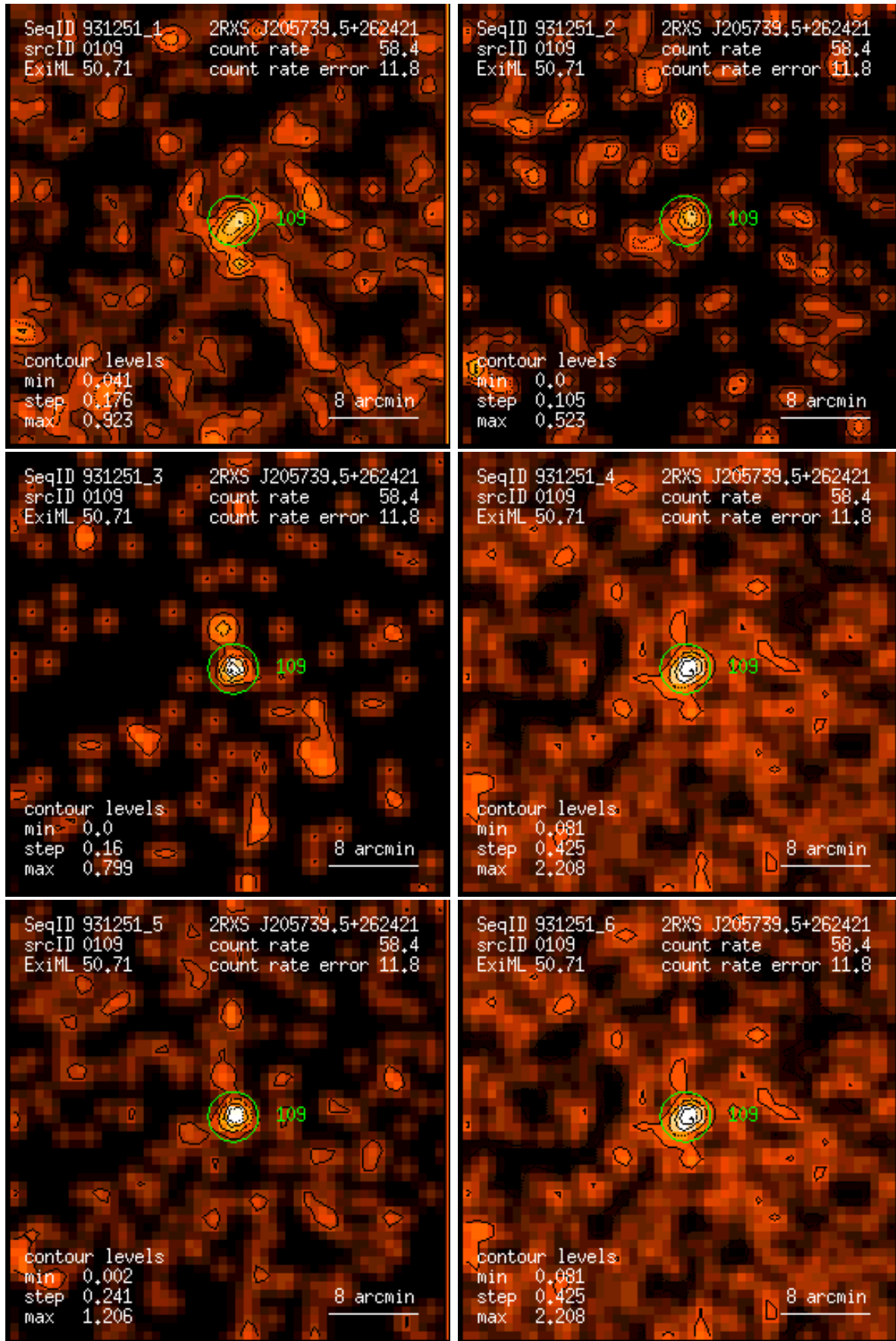
Figure 109: RASS 931251: detection 0109: band rate images, Gaussian filter: (1) PSPC channels 11 – 41, (2) 52 – 90, (3) 91 – 201, (4) 11 – 235, (5) 52 – 201, (6) 11 – 201. Broad band rates in counts/ks. Band rate contour levels in counts/ks/arcmin 2 .
