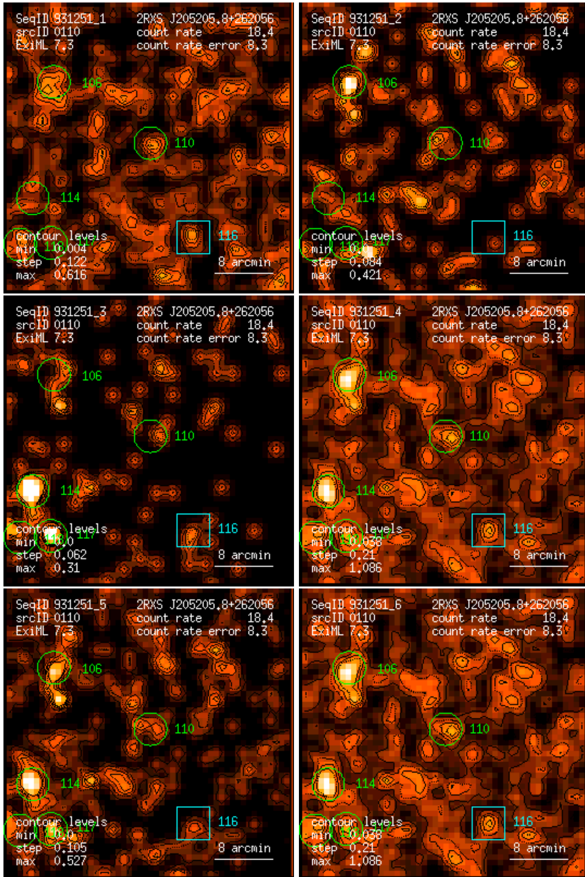
Figure 110: RASS 931251: detection 0110: band rate images, Gaussian filter: (1) PSPC channels 11 – 41, (2) 52 – 90, (3) 91 – 201, (4) 11 – 235, (5) 52 – 201, (6) 11 – 201. Broad band rates in counts/ks. Band rate contour levels in counts/ks/arcmin 2 .
