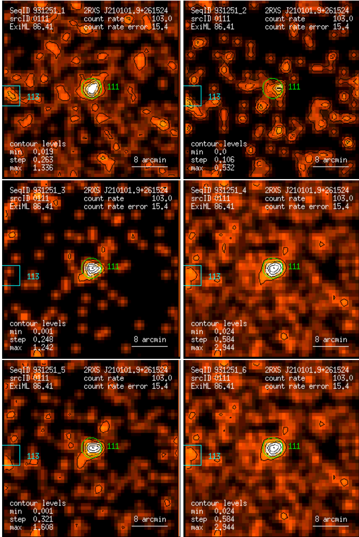
Figure 111: RASS 931251: detection 0111: band rate images, Gaussian filter: (1) PSPC channels 11 – 41, (2) 52 – 90, (3) 91 – 201, (4) 11 – 235, (5) 52 – 201, (6) 11 – 201. Broad band rates in counts/ks. Band rate contour levels in counts/ks/arcmin 2 .
