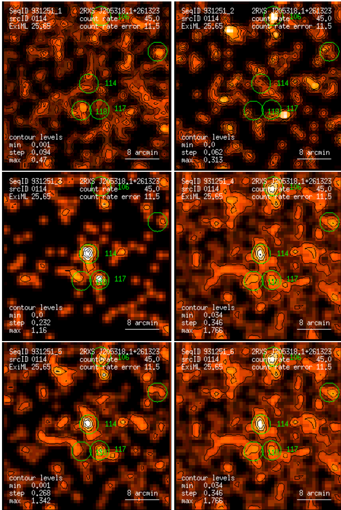
Figure 114: RASS 931251: detection 0114: band rate images, Gaussian filter: (1) PSPC channels 11 – 41, (2) 52 – 90, (3) 91 – 201, (4) 11 – 235, (5) 52 – 201, (6) 11 – 201. Broad band rates in counts/ks. Band rate contour levels in counts/ks/arcmin 2 .
