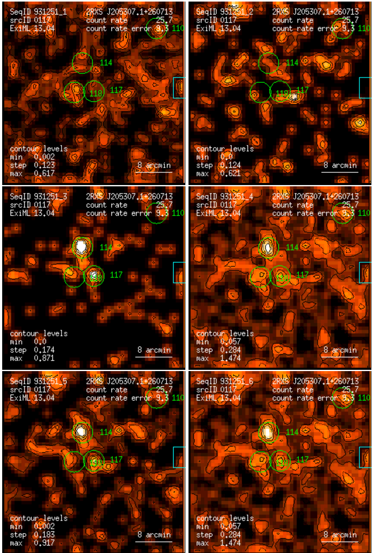
Figure 117: RASS 931251: detection 0117: band rate images, Gaussian filter: (1) PSPC channels 11 – 41, (2) 52 – 90, (3) 91 – 201, (4) 11 – 235, (5) 52 – 201, (6) 11 – 201. Broad band rates in counts/ks. Band rate contour levels in counts/ks/arcmin 2 .
