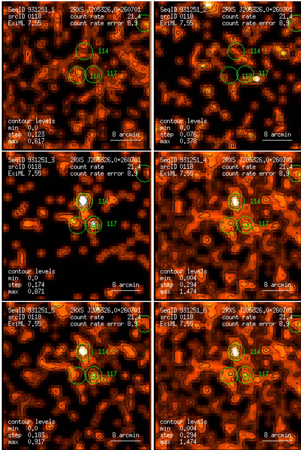
Figure 118: RASS 931251: detection 0118: band rate images, Gaussian filter: (1) PSPC channels 11 – 41, (2) 52 – 90, (3) 91 – 201, (4) 11 – 235, (5) 52 – 201, (6) 11 – 201. Broad band rates in counts/ks. Band rate contour levels in counts/ks/arcmin 2 .
