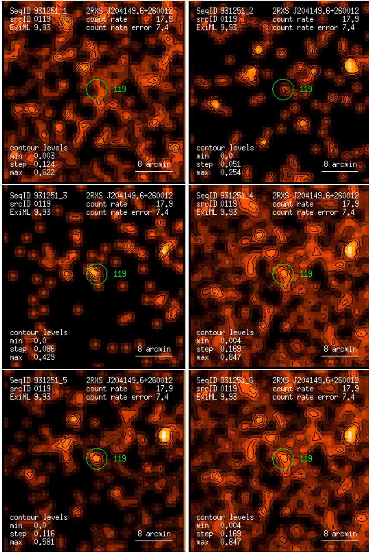
Figure 119: RASS 931251: detection 0119: band rate images, Gaussian filter: (1) PSPC channels 11 – 41, (2) 52 – 90, (3) 91 – 201, (4) 11 – 235, (5) 52 – 201, (6) 11 – 201. Broad band rates in counts/ks. Band rate contour levels in counts/ks/arcmin 2 .
