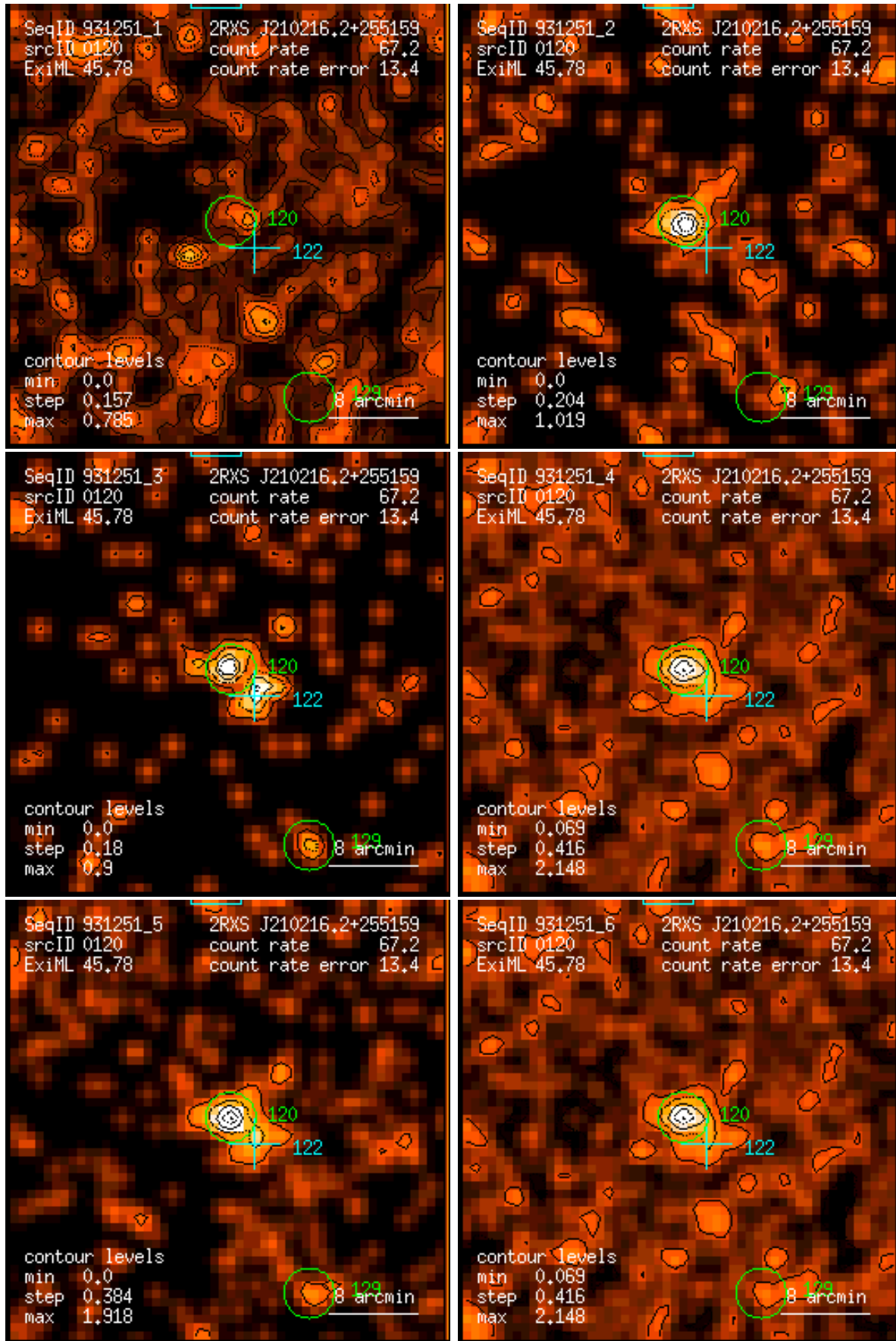
Figure 120: RASS 931251: detection 0120: band rate images, Gaussian filter: (1) PSPC channels 11 – 41, (2) 52 – 90, (3) 91 – 201, (4) 11 – 235, (5) 52 – 201, (6) 11 – 201. Broad band rates in counts/ks. Band rate contour levels in counts/ks/arcmin 2 .
