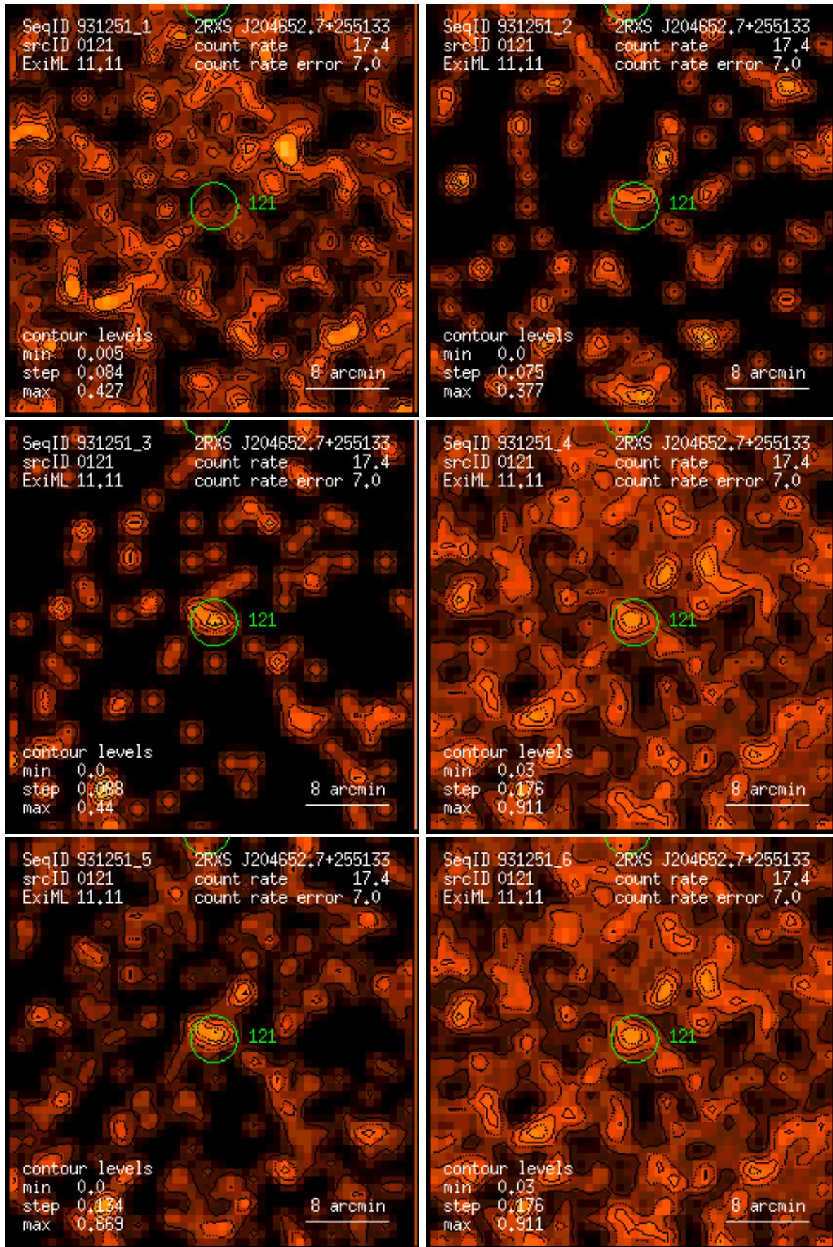
Figure 121: RASS 931251: detection 0121: band rate images, Gaussian filter: (1) PSPC channels 11 – 41, (2) 52 – 90, (3) 91 – 201, (4) 11 – 235, (5) 52 – 201, (6) 11 – 201. Broad band rates in counts/ks. Band rate contour levels in counts/ks/arcmin 2 .
