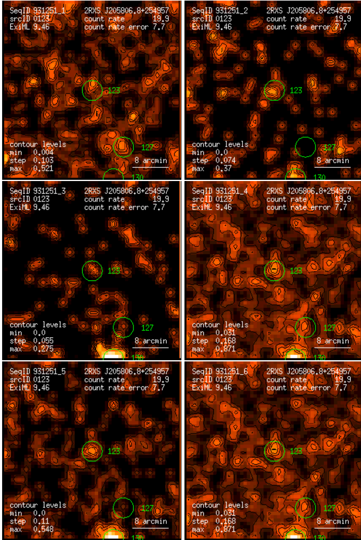
Figure 123: RASS 931251: detection 0123: band rate images, Gaussian filter: (1) PSPC channels 11 – 41, (2) 52 – 90, (3) 91 – 201, (4) 11 – 235, (5) 52 – 201, (6) 11 – 201. Broad band rates in counts/ks. Band rate contour levels in counts/ks/arcmin 2 .
