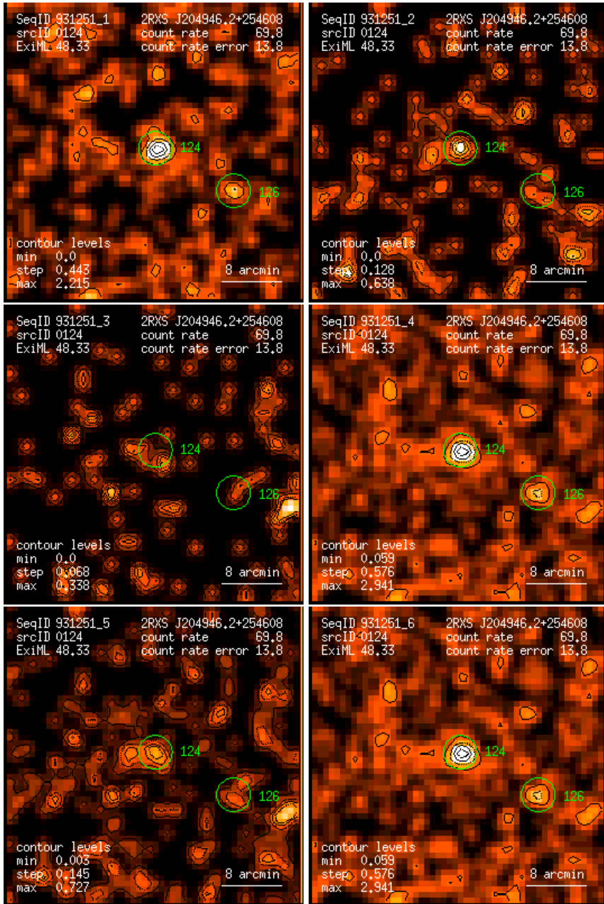
Figure 124: RASS 931251: detection 0124: band rate images, Gaussian filter: (1) PSPC channels 11 – 41, (2) 52 – 90, (3) 91 – 201, (4) 11 – 235, (5) 52 – 201, (6) 11 – 201. Broad band rates in counts/ks. Band rate contour levels in counts/ks/arcmin 2 .
