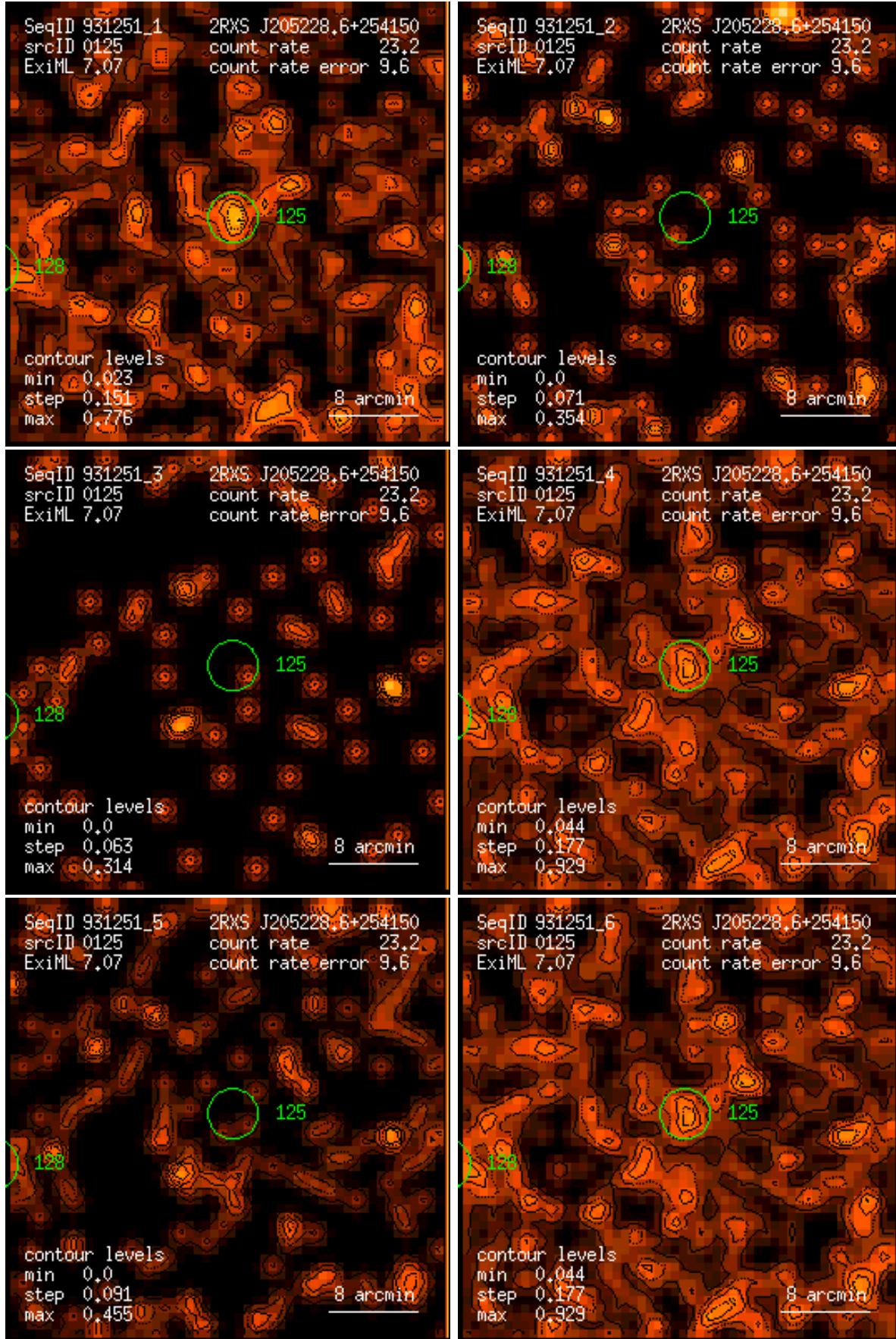
Figure 125: RASS 931251: detection 0125: band rate images, Gaussian filter: (1) PSPC channels 11 – 41, (2) 52 – 90, (3) 91 – 201, (4) 11 – 235, (5) 52 – 201, (6) 11 – 201. Broad band rates in counts/ks. Band rate contour levels in counts/ks/arcmin 2 .
