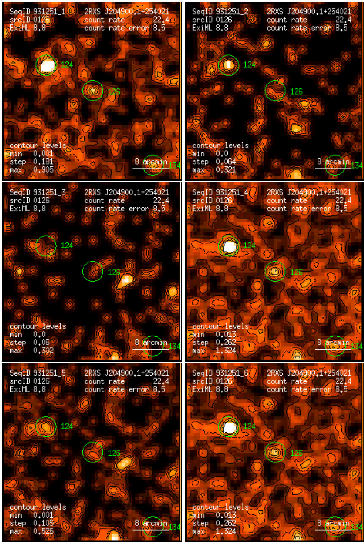
Figure 126: RASS 931251: detection 0126: band rate images, Gaussian filter: (1) PSPC channels 11 – 41, (2) 52 – 90, (3) 91 – 201, (4) 11 – 235, (5) 52 – 201, (6) 11 – 201. Broad band rates in counts/ks. Band rate contour levels in counts/ks/arcmin 2 .
