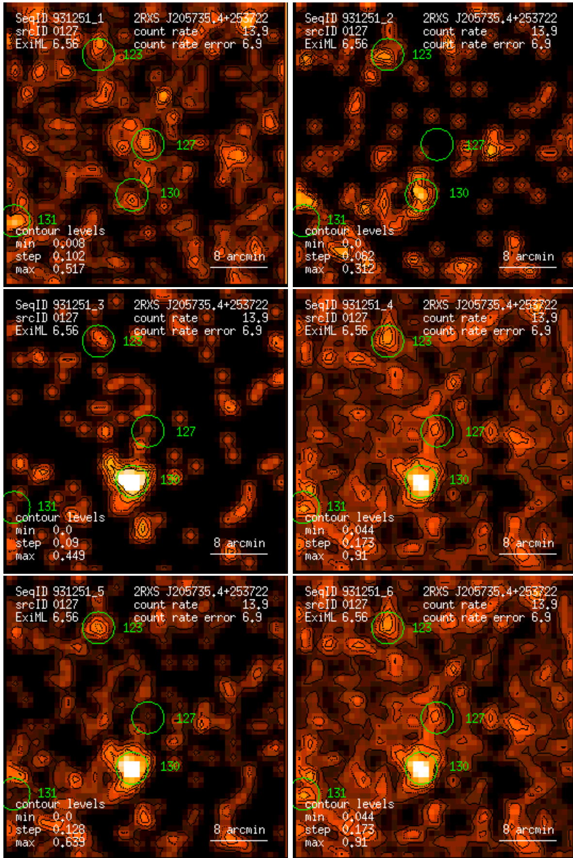
Figure 127: RASS 931251: detection 0127: band rate images, Gaussian filter: (1) PSPC channels 11 – 41, (2) 52 – 90, (3) 91 – 201, (4) 11 – 235, (5) 52 – 201, (6) 11 – 201. Broad band rates in counts/ks. Band rate contour levels in counts/ks/arcmin 2 .
