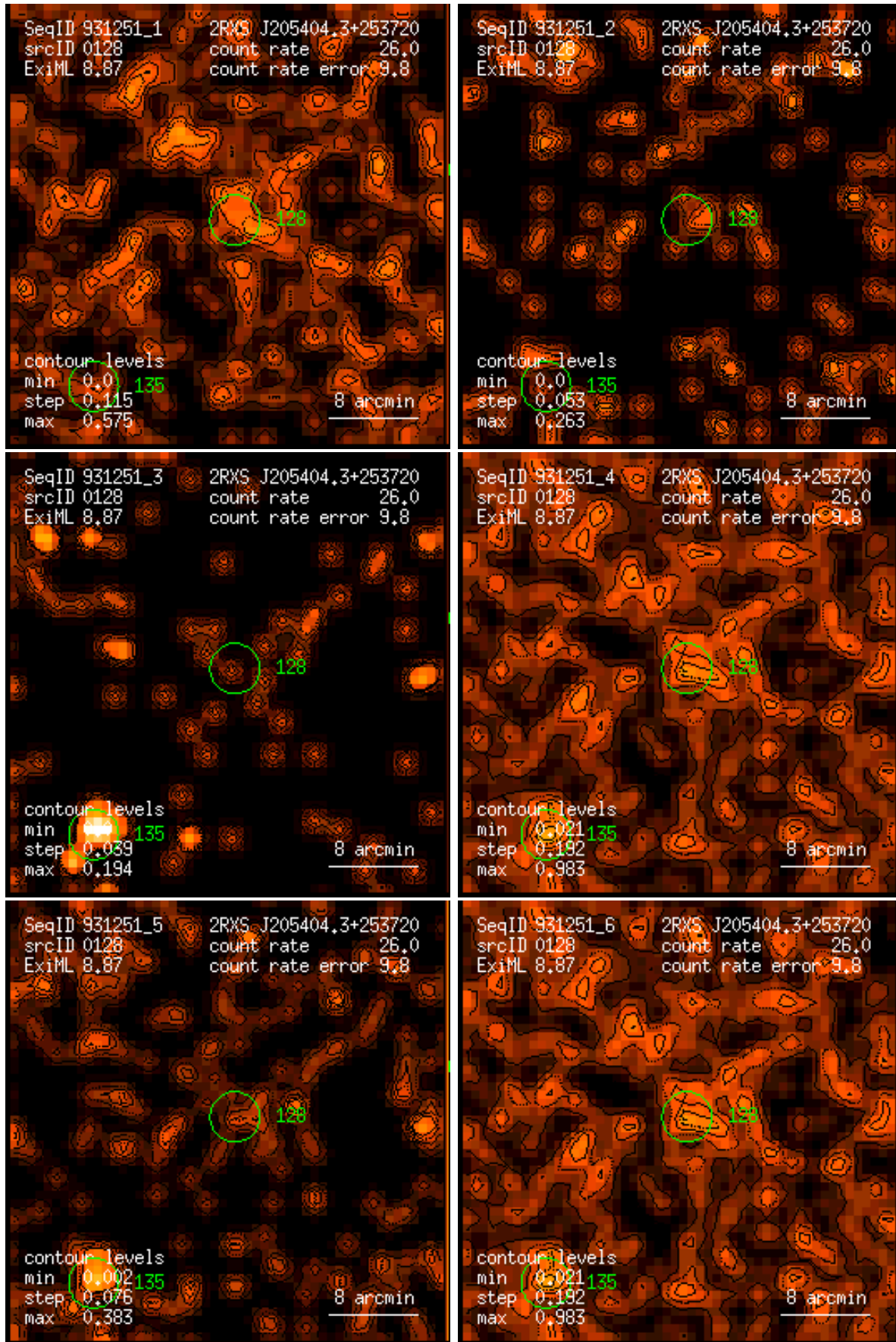
Figure 128: RASS 931251: detection 0128: band rate images, Gaussian filter: (1) PSPC channels 11 – 41, (2) 52 – 90, (3) 91 – 201, (4) 11 – 235, (5) 52 – 201, (6) 11 – 201. Broad band rates in counts/ks. Band rate contour levels in counts/ks/arcmin 2 .
