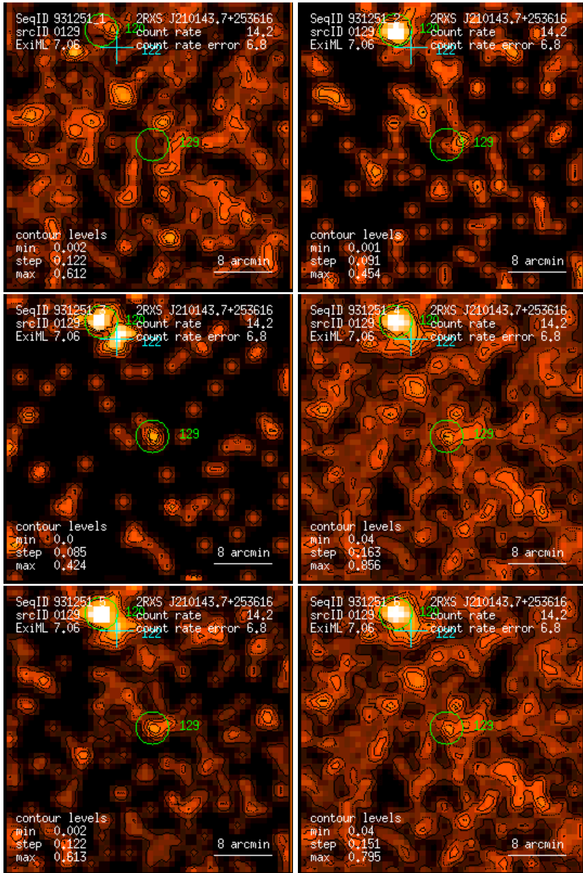
Figure 129: RASS 931251: detection 0129: band rate images, Gaussian filter: (1) PSPC channels 11 – 41, (2) 52 – 90, (3) 91 – 201, (4) 11 – 235, (5) 52 – 201, (6) 11 – 201. Broad band rates in counts/ks. Band rate contour levels in counts/ks/arcmin 2 .
