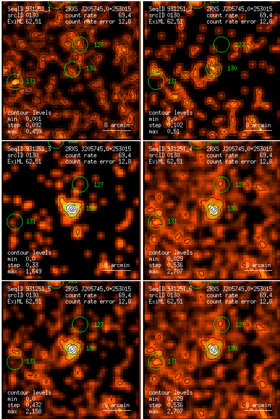
Figure 130: RASS 931251: detection 0130: band rate images, Gaussian filter: (1) PSPC channels 11 – 41, (2) 52 – 90, (3) 91 – 201, (4) 11 – 235, (5) 52 – 201, (6) 11 – 201. Broad band rates in counts/ks. Band rate contour levels in counts/ks/arcmin 2 .
