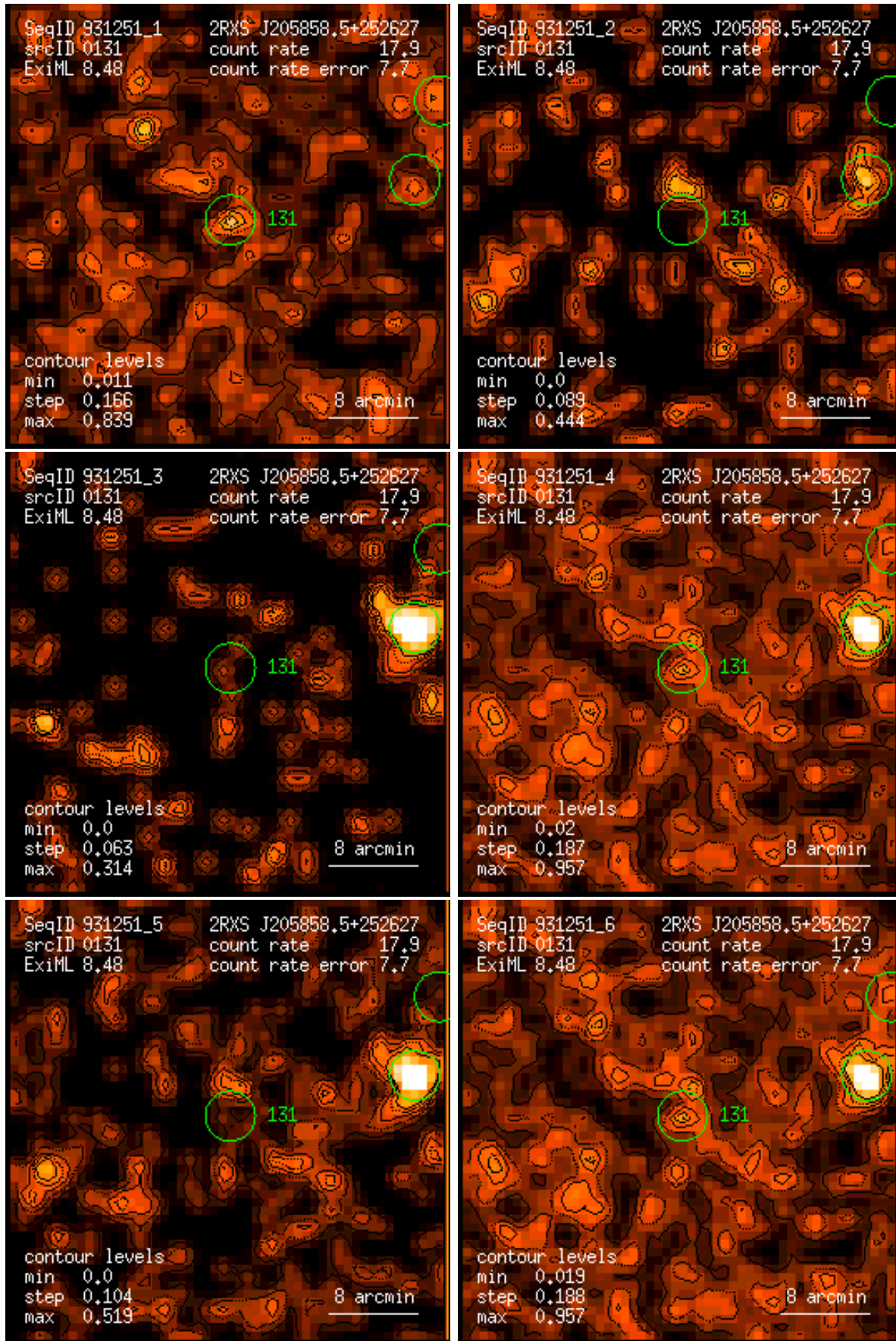
Figure 131: RASS 931251: detection 0131: band rate images, Gaussian filter: (1) PSPC channels 11 – 41, (2) 52 – 90, (3) 91 – 201, (4) 11 – 235, (5) 52 – 201, (6) 11 – 201. Broad band rates in counts/ks. Band rate contour levels in counts/ks/arcmin 2 .
