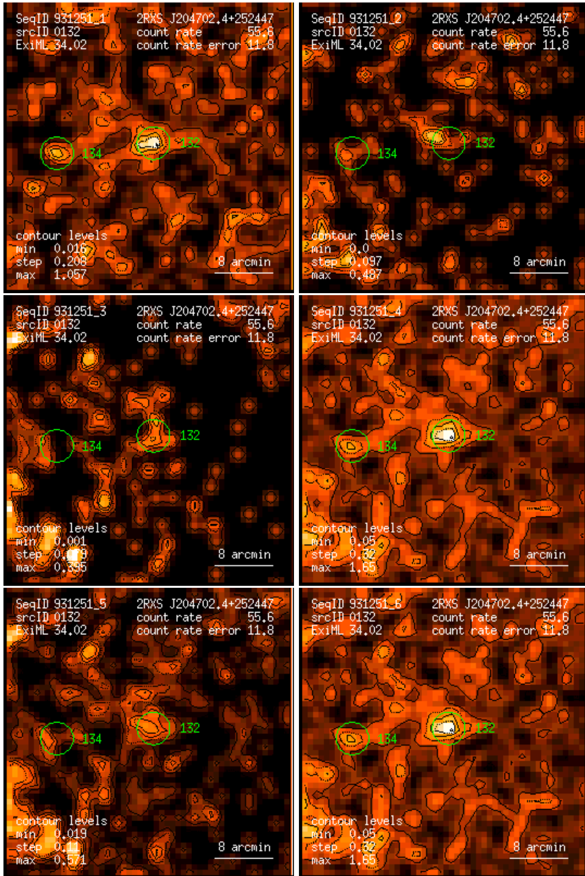
Figure 132: RASS 931251: detection 0132: band rate images, Gaussian filter: (1) PSPC channels 11 – 41, (2) 52 – 90, (3) 91 – 201, (4) 11 – 235, (5) 52 – 201, (6) 11 – 201. Broad band rates in counts/ks. Band rate contour levels in counts/ks/arcmin 2 .
