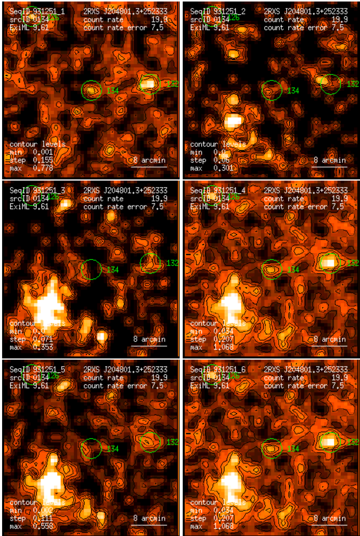
Figure 134: RASS 931251: detection 0134: band rate images, Gaussian filter: (1) PSPC channels 11 – 41, (2) 52 – 90, (3) 91 – 201, (4) 11 – 235, (5) 52 – 201, (6) 11 – 201. Broad band rates in counts/ks. Band rate contour levels in counts/ks/arcmin 2 .
