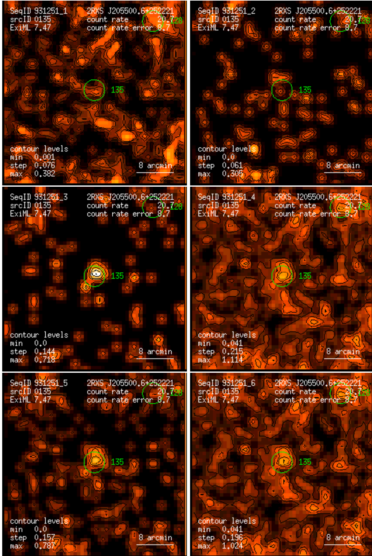
Figure 135: RASS 931251: detection 0135: band rate images, Gaussian filter: (1) PSPC channels 11 – 41, (2) 52 – 90, (3) 91 – 201, (4) 11 – 235, (5) 52 – 201, (6) 11 – 201. Broad band rates in counts/ks. Band rate contour levels in counts/ks/arcmin 2 .
