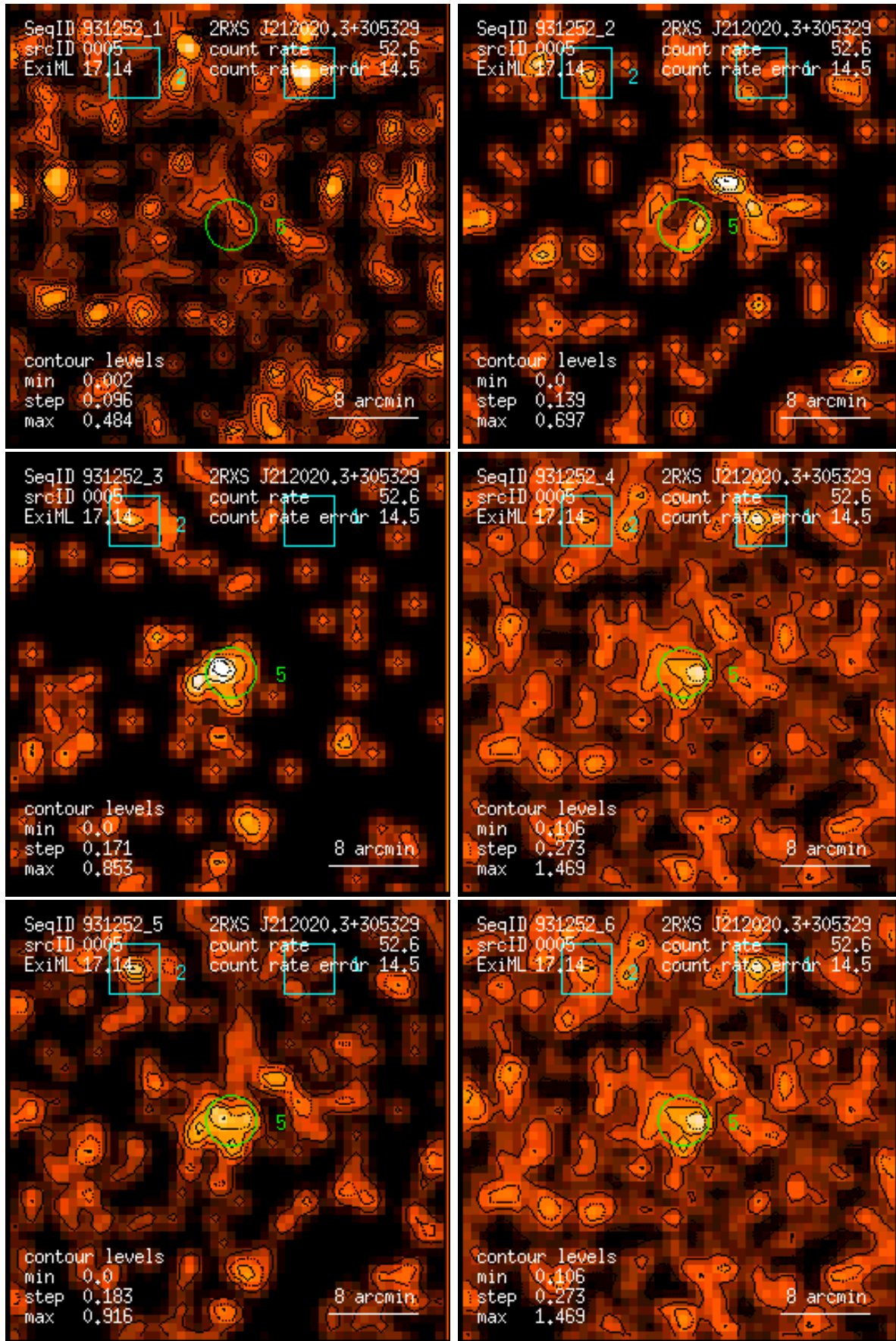
Figure 5: RASS 931252: detection 0005: band rate images, Gaussian filter: (1) PSPC channels 11 – 41, (2) 52 – 90, (3) 91 – 201, (4) 11 – 235, (5) 52 – 201, (6) 11 – 201. Broad band rates in counts/ks. Band rate contour levels in counts/ks/arcmin 2 .
