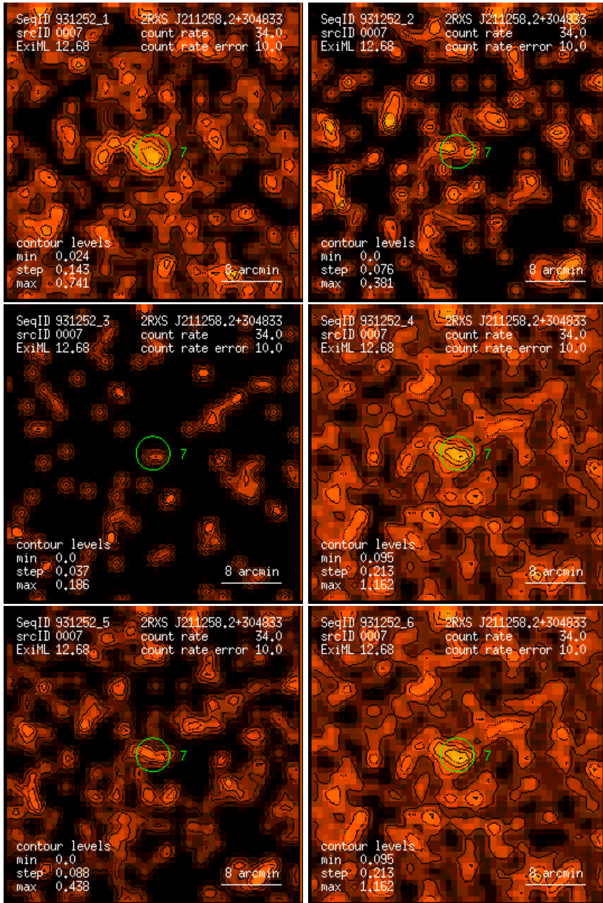
Figure 7: RASS 931252: detection 0007: band rate images, Gaussian filter: (1) PSPC channels 11 – 41, (2) 52 – 90, (3) 91 – 201, (4) 11 – 235, (5) 52 – 201, (6) 11 – 201. Broad band rates in counts/ks. Band rate contour levels in counts/ks/arcmin 2 .
