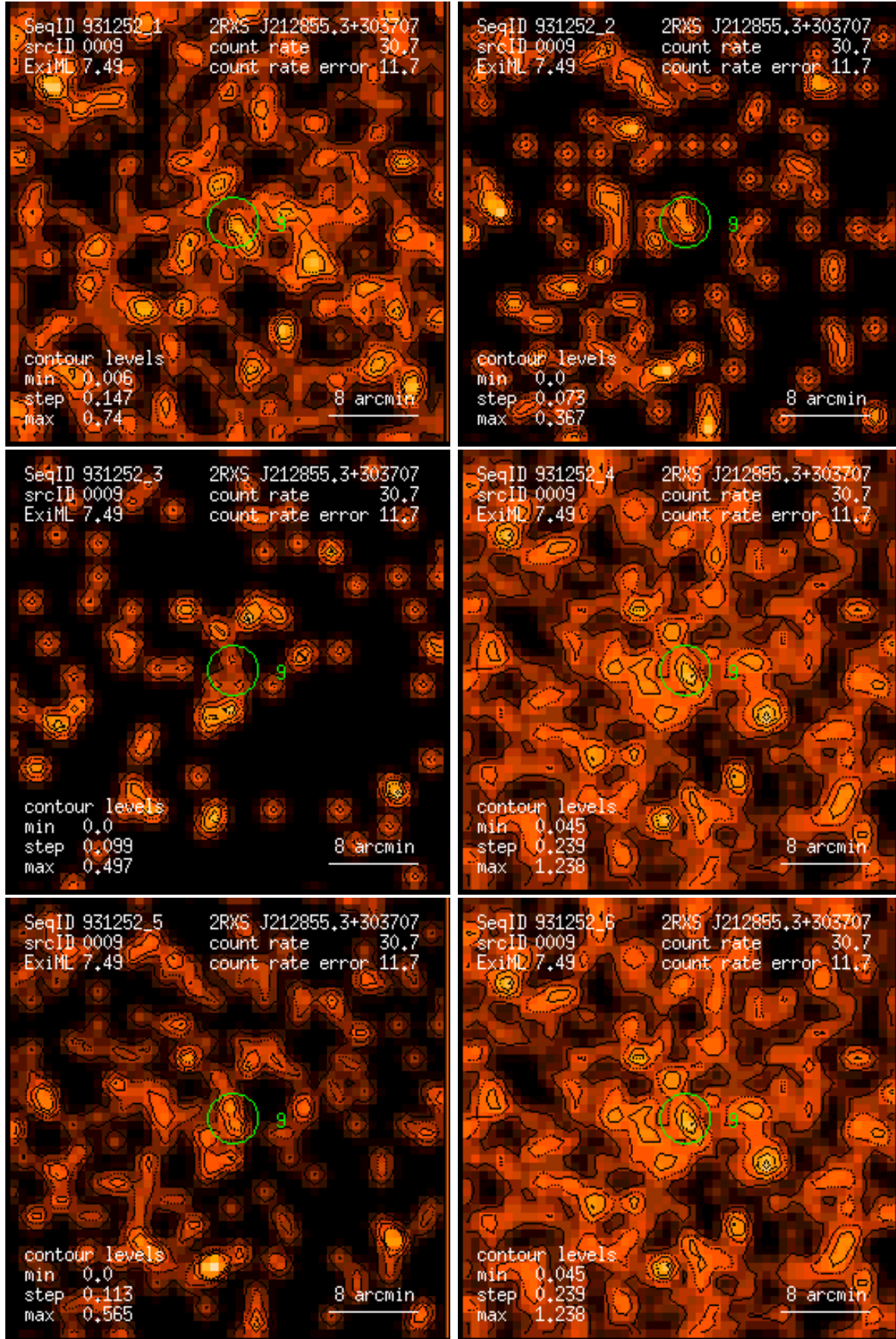
Figure 9: RASS 931252: detection 0009: band rate images, Gaussian filter: (1) PSPC channels 11 – 41, (2) 52 – 90, (3) 91 – 201, (4) 11 – 235, (5) 52 – 201, (6) 11 – 201. Broad band rates in counts/ks. Band rate contour levels in counts/ks/arcmin 2 .
