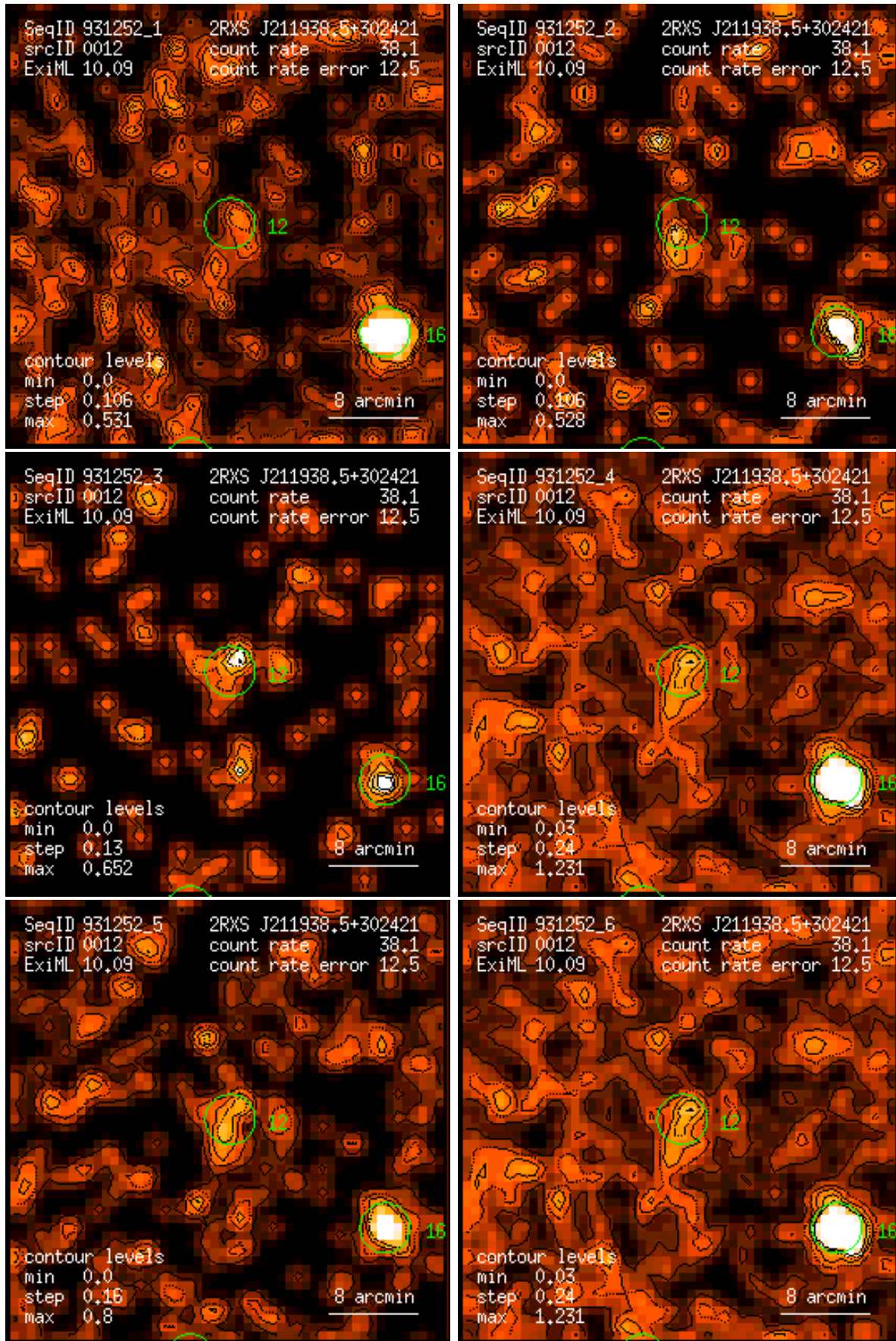
Figure 12: RASS 931252: detection 0012: band rate images, Gaussian filter: (1) PSPC channels 11 – 41, (2) 52 – 90, (3) 91 – 201, (4) 11 – 235, (5) 52 – 201, (6) 11 – 201. Broad band rates in counts/ks. Band rate contour levels in counts/ks/arcmin 2 .
