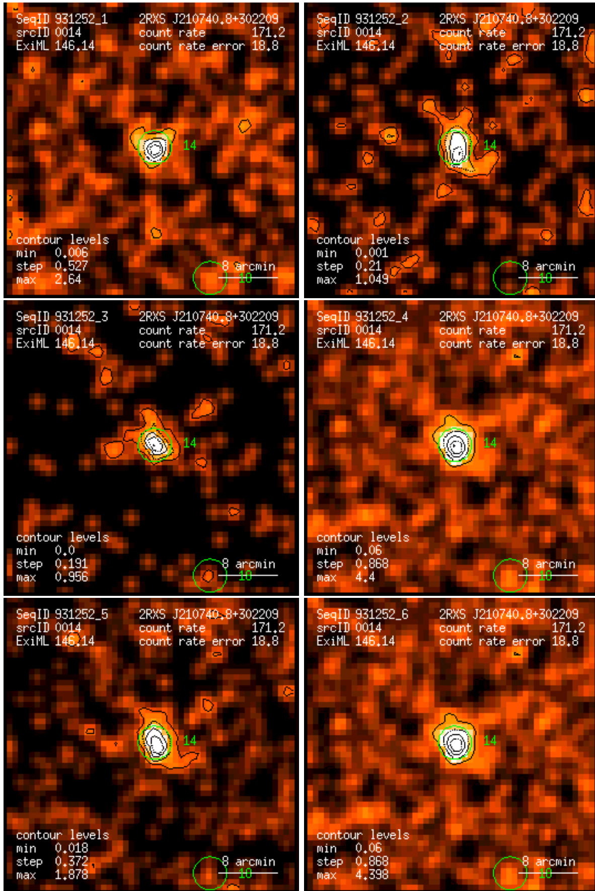
Figure 14: RASS 931252: detection 0014: band rate images, Gaussian filter: (1) PSPC channels 11 – 41, (2) 52 – 90, (3) 91 – 201, (4) 11 – 235, (5) 52 – 201, (6) 11 – 201. Broad band rates in counts/ks. Band rate contour levels in counts/ks/arcmin 2 .
