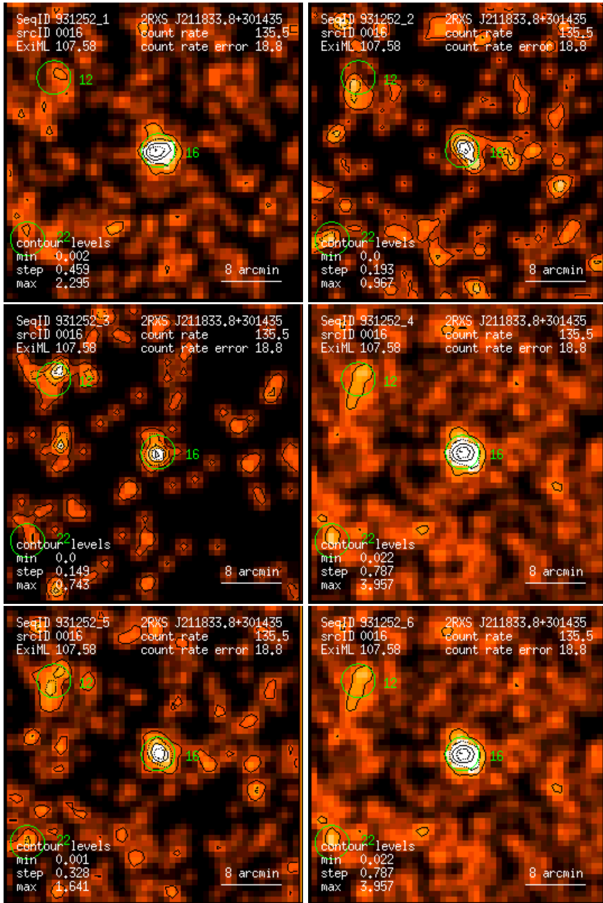
Figure 16: RASS 931252: detection 0016: band rate images, Gaussian filter: (1) PSPC channels 11 – 41, (2) 52 – 90, (3) 91 – 201, (4) 11 – 235, (5) 52 – 201, (6) 11 – 201. Broad band rates in counts/ks. Band rate contour levels in counts/ks/arcmin 2 .
