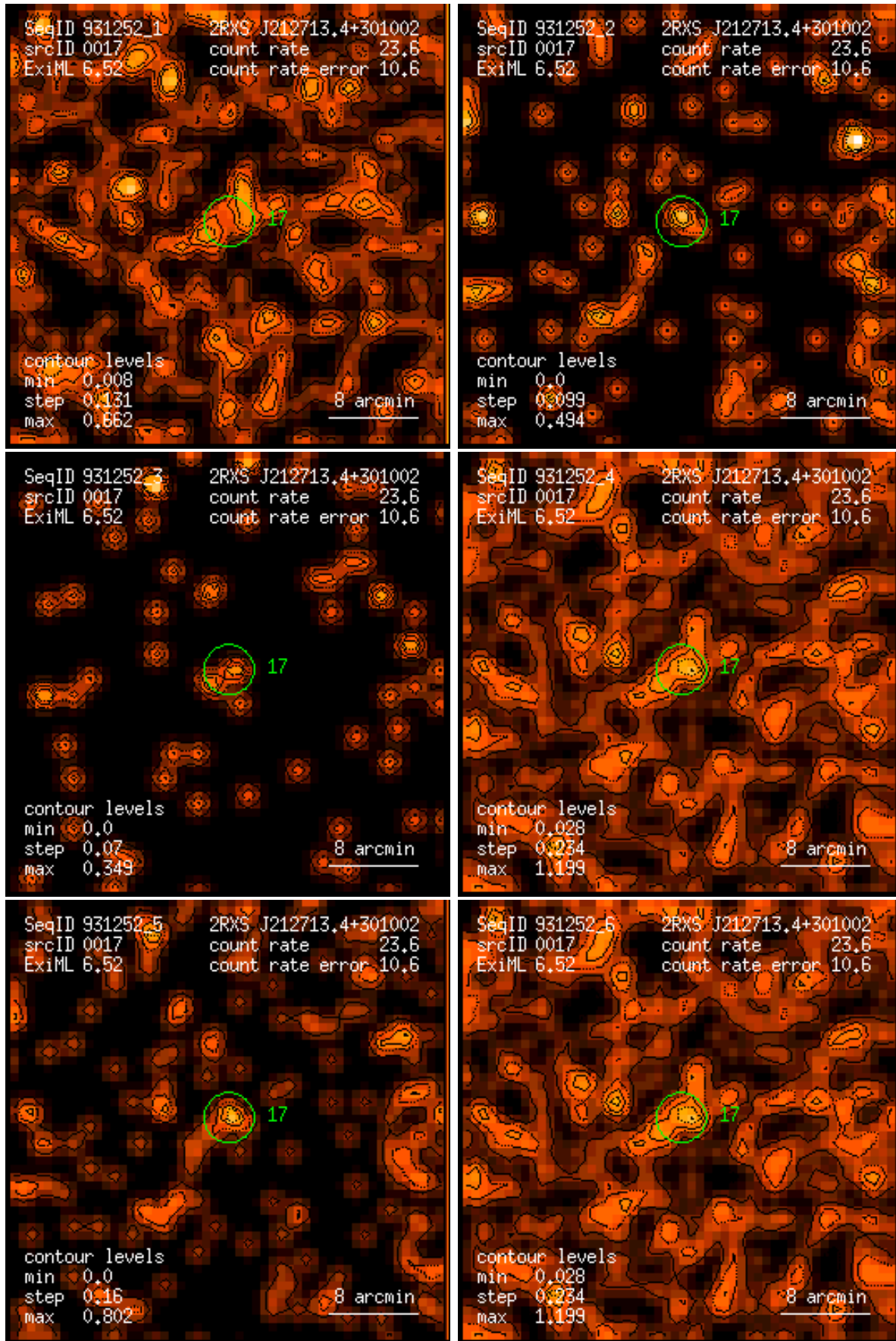
Figure 17: RASS 931252: detection 0017: band rate images, Gaussian filter: (1) PSPC channels 11 – 41, (2) 52 – 90, (3) 91 – 201, (4) 11 – 235, (5) 52 – 201, (6) 11 – 201. Broad band rates in counts/ks. Band rate contour levels in counts/ks/arcmin 2 .
