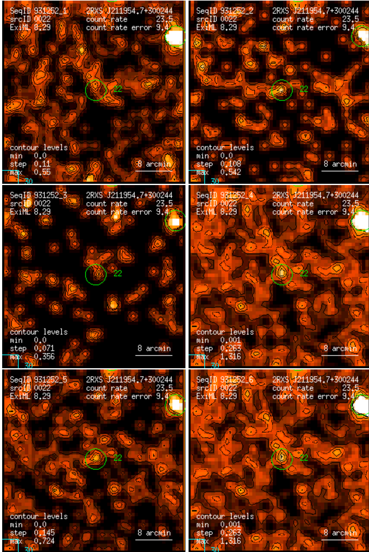
Figure 22: RASS 931252: detection 0022: band rate images, Gaussian filter: (1) PSPC channels 11 – 41, (2) 52 – 90, (3) 91 – 201, (4) 11 – 235, (5) 52 – 201, (6) 11 – 201. Broad band rates in counts/ks. Band rate contour levels in counts/ks/arcmin 2 .
