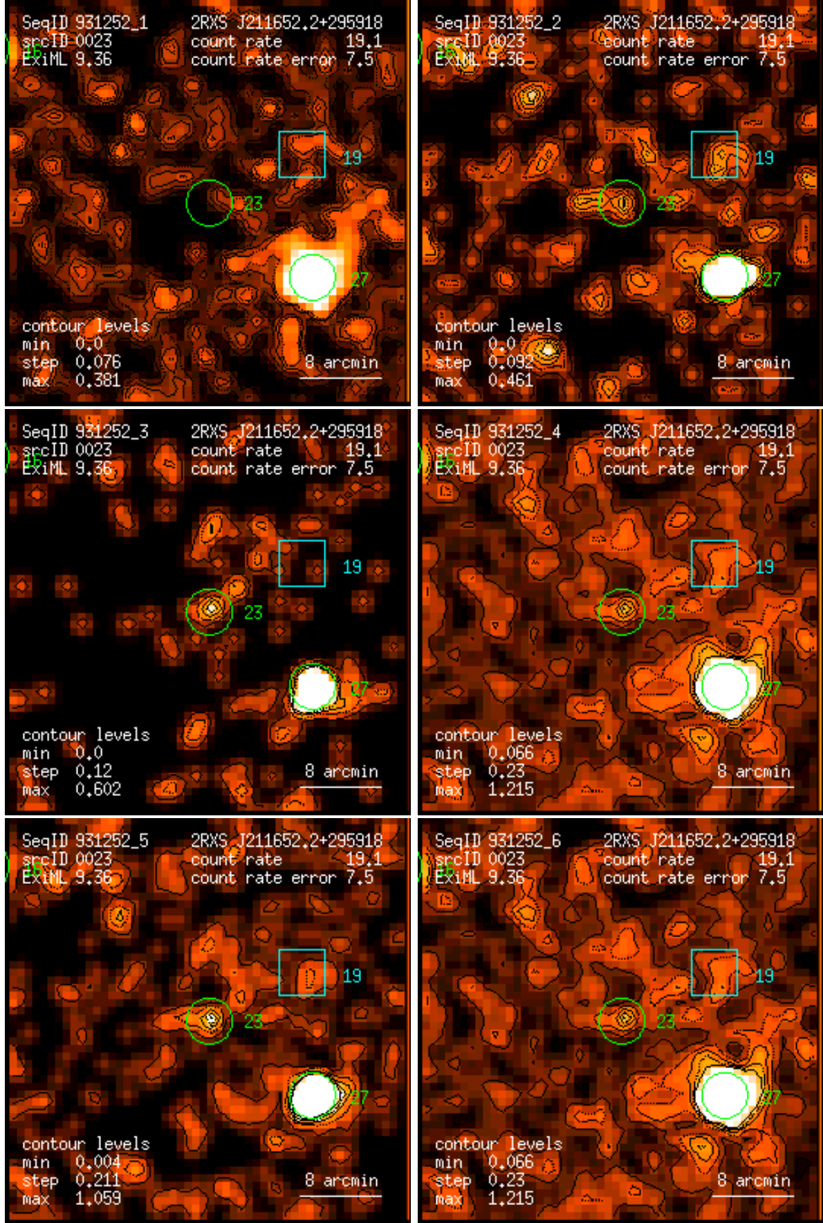
Figure 23: RASS 931252: detection 0023: band rate images, Gaussian filter: (1) PSPC channels 11 – 41, (2) 52 – 90, (3) 91 – 201, (4) 11 – 235, (5) 52 – 201, (6) 11 – 201. Broad band rates in counts/ks. Band rate contour levels in counts/ks/arcmin 2 .
