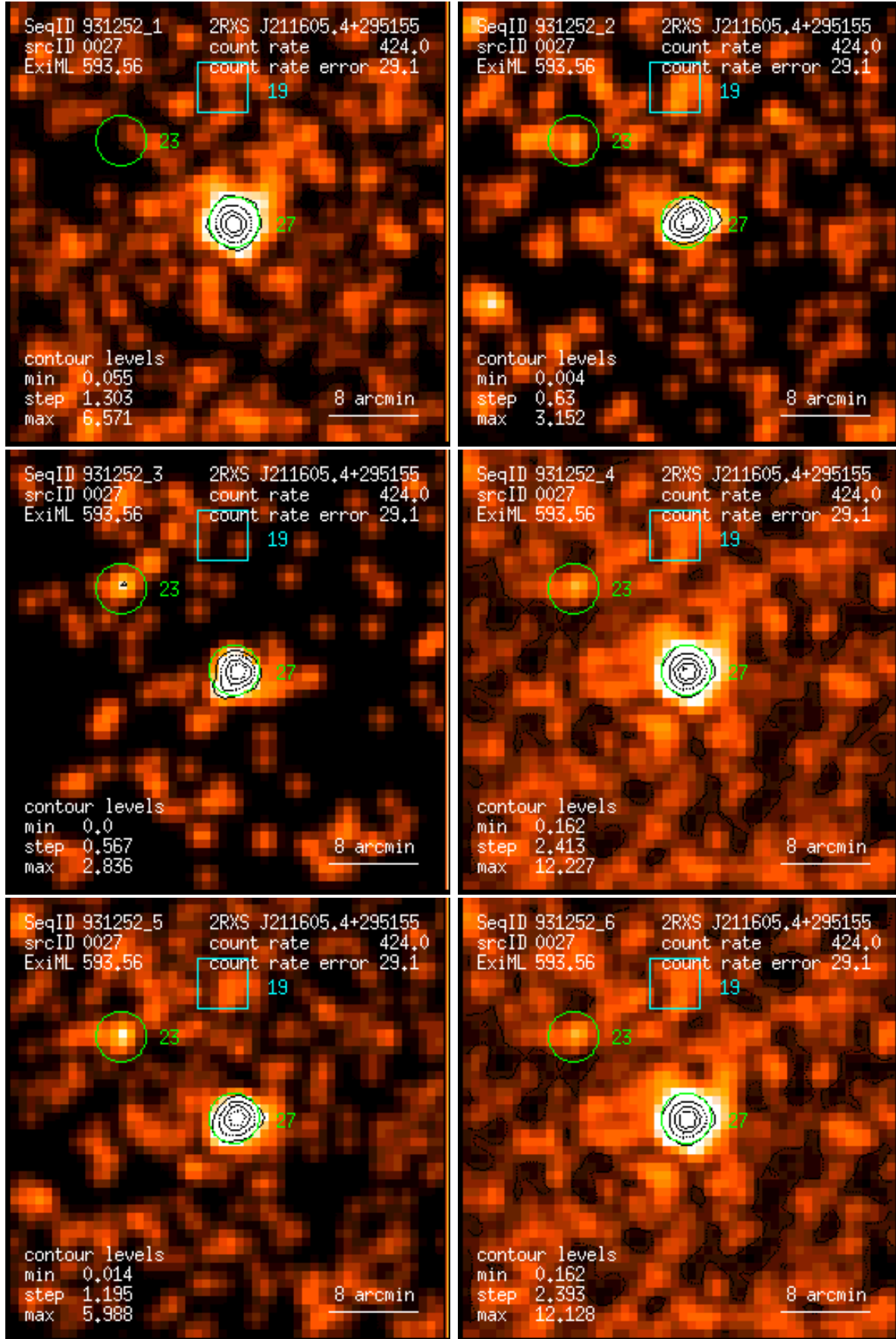
Figure 27: RASS 931252: detection 0027: band rate images, Gaussian filter: (1) PSPC channels 11 – 41, (2) 52 – 90, (3) 91 – 201, (4) 11 – 235, (5) 52 – 201, (6) 11 – 201. Broad band rates in counts/ks. Band rate contour levels in counts/ks/arcmin 2 .
