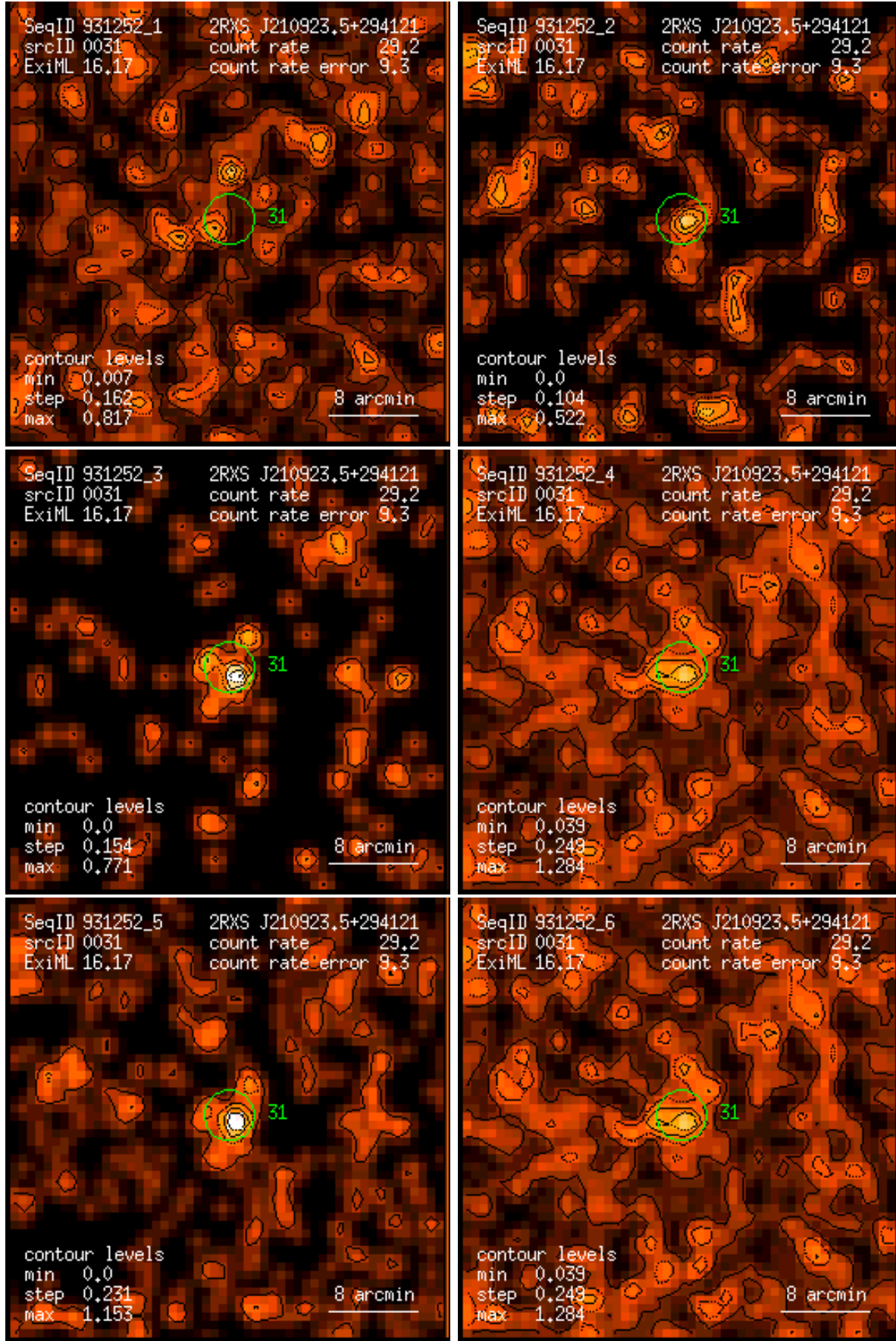
Figure 31: RASS 931252: detection 0031: band rate images, Gaussian filter: (1) PSPC channels 11 – 41, (2) 52 – 90, (3) 91 – 201, (4) 11 – 235, (5) 52 – 201, (6) 11 – 201. Broad band rates in counts/ks. Band rate contour levels in counts/ks/arcmin 2 .
