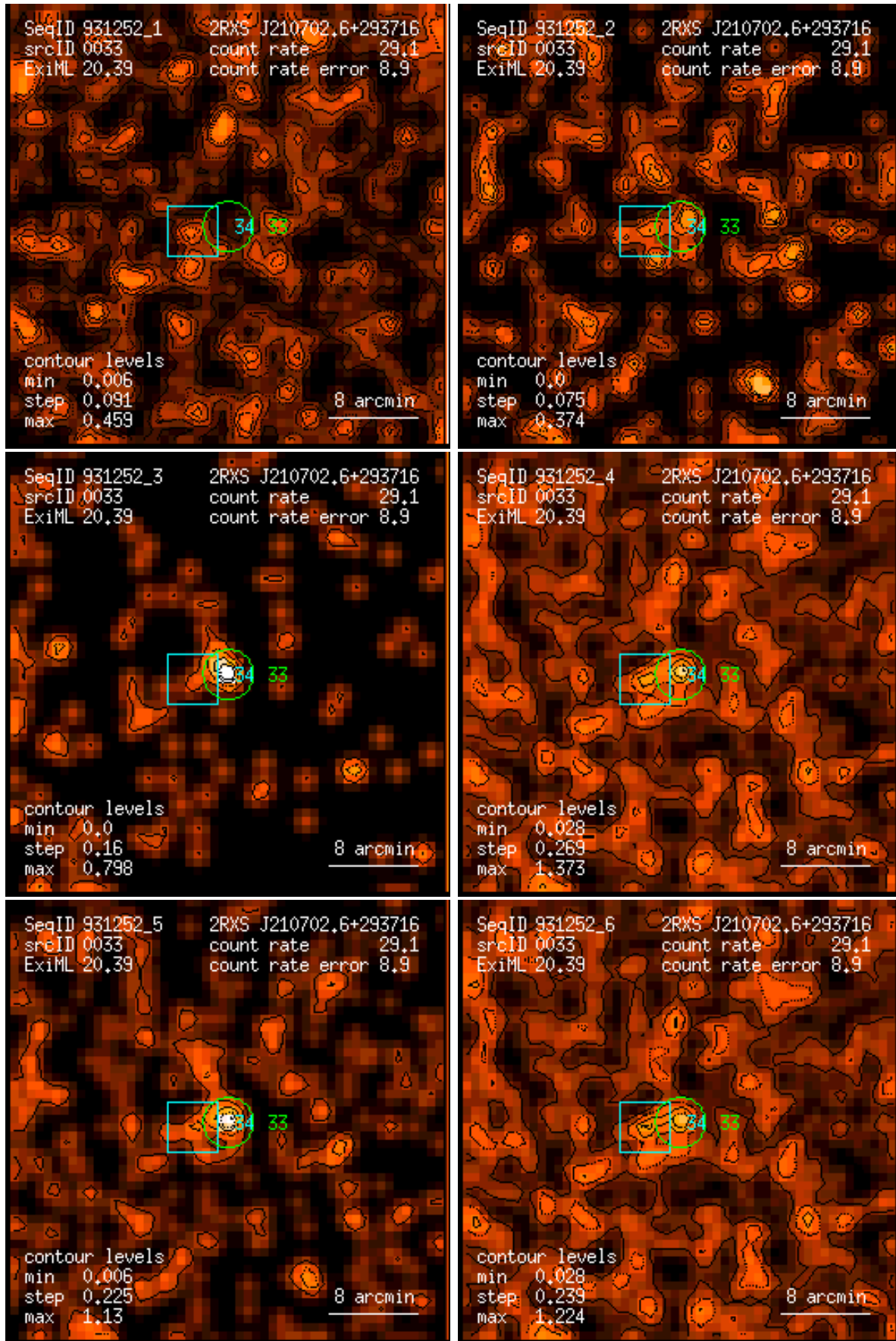
Figure 33: RASS 931252: detection 0033: band rate images, Gaussian filter: (1) PSPC channels 11 – 41, (2) 52 – 90, (3) 91 – 201, (4) 11 – 235, (5) 52 – 201, (6) 11 – 201. Broad band rates in counts/ks. Band rate contour levels in counts/ks/arcmin 2 .
