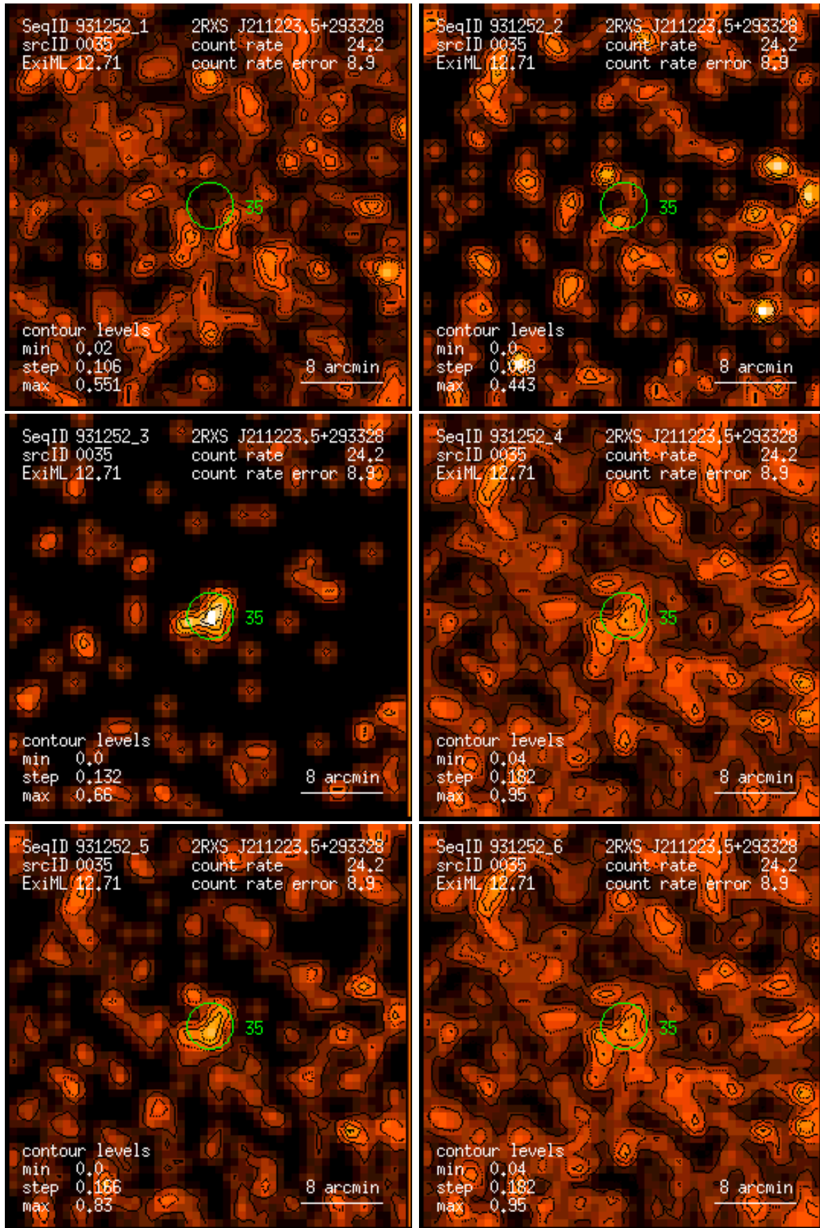
Figure 35: RASS 931252: detection 0035: band rate images, Gaussian filter: (1) PSPC channels 11 – 41, (2) 52 – 90, (3) 91 – 201, (4) 11 – 235, (5) 52 – 201, (6) 11 – 201. Broad band rates in counts/ks. Band rate contour levels in counts/ks/arcmin 2 .
