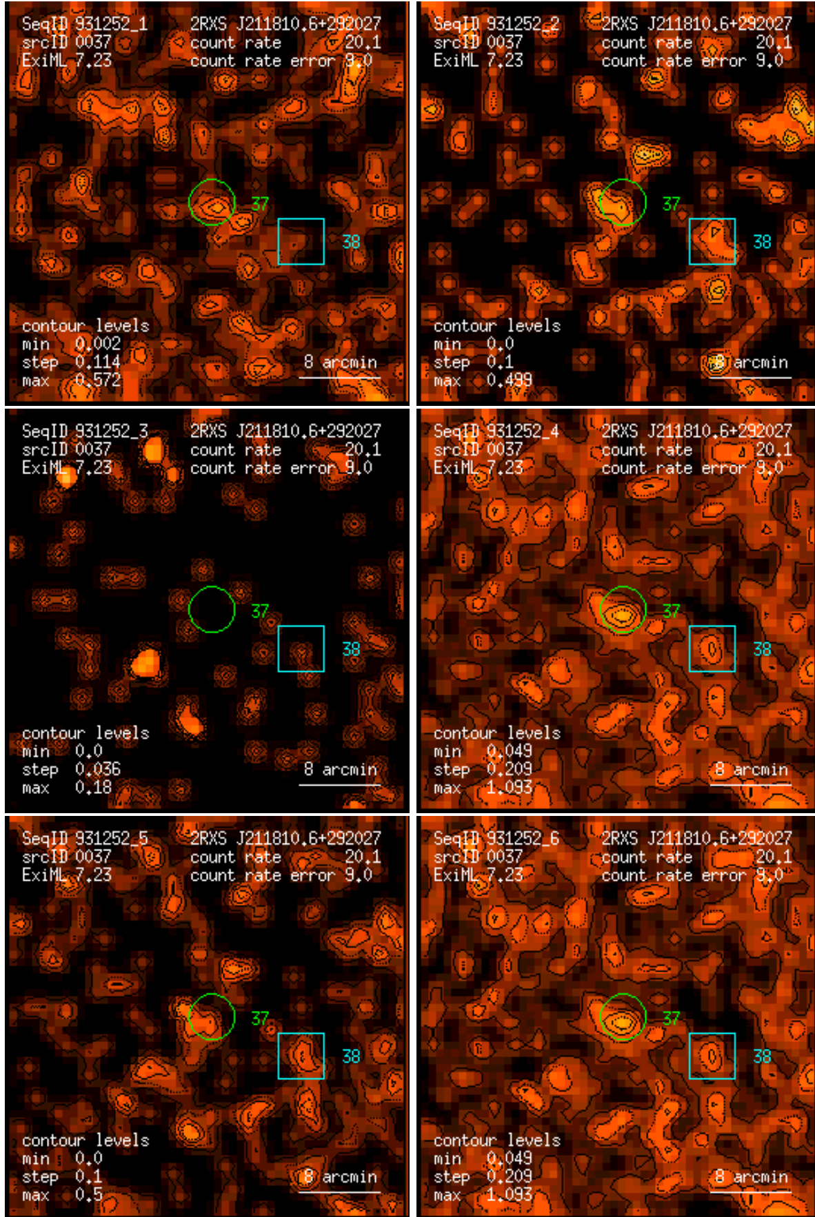
Figure 37: RASS 931252: detection 0037: band rate images, Gaussian filter: (1) PSPC channels 11 – 41, (2) 52 – 90, (3) 91 – 201, (4) 11 – 235, (5) 52 – 201, (6) 11 – 201. Broad band rates in counts/ks. Band rate contour levels in counts/ks/arcmin 2 .
