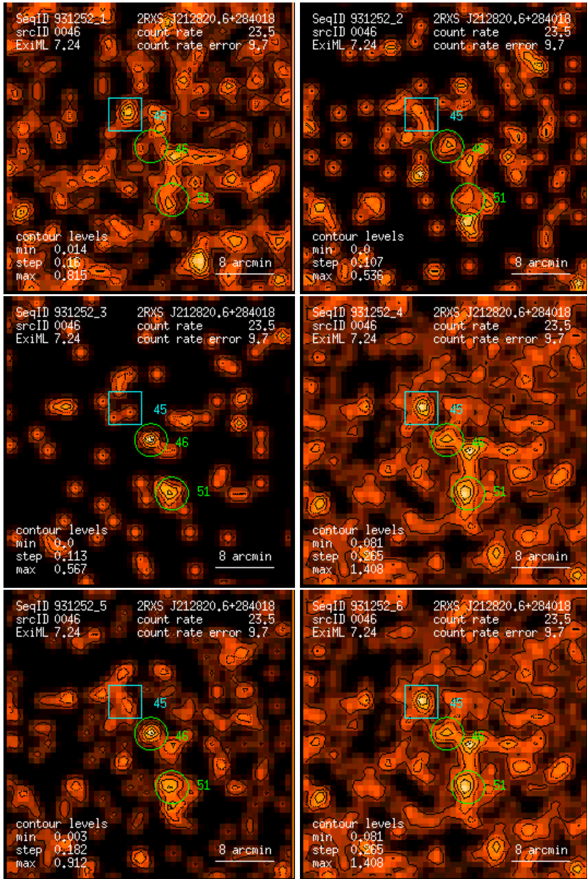
Figure 46: RASS 931252: detection 0046: band rate images, Gaussian filter: (1) PSPC channels 11 – 41, (2) 52 – 90, (3) 91 – 201, (4) 11 – 235, (5) 52 – 201, (6) 11 – 201. Broad band rates in counts/ks. Band rate contour levels in counts/ks/arcmin 2 .
