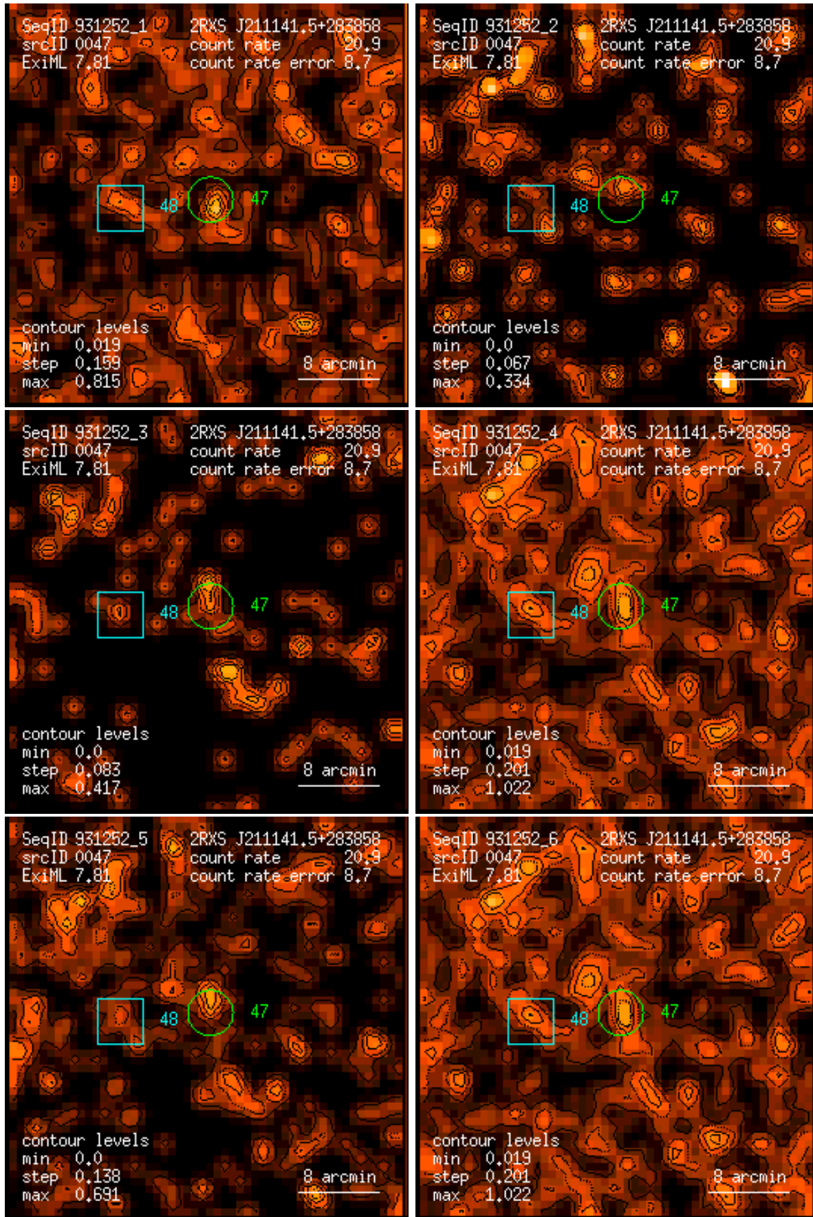
Figure 47: RASS 931252: detection 0047: band rate images, Gaussian filter: (1) PSPC channels 11 – 41, (2) 52 – 90, (3) 91 – 201, (4) 11 – 235, (5) 52 – 201, (6) 11 – 201. Broad band rates in counts/ks. Band rate contour levels in counts/ks/arcmin 2 .
